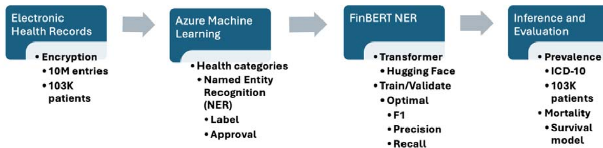
Figure 1. Workflow of the study. Textual electronic health records (EHRs) were encrypted and scrubbed of all personal information. Working with domain experts, we applied keywords to identify relevant EHR entries and performed appropriate subsampling for labelling within Azure Machine Learning Studio. FinBERT library, a pretrained BERT model adopted for the Finnish language, and the Hugging Face-associated transformer libraries were integrated for the processing, training, and evaluation of the labelled and approved EHR text data. Abbreviations: ICD-10, International Classification of Diseases, 10 th Revision; NER, named entity recognition
