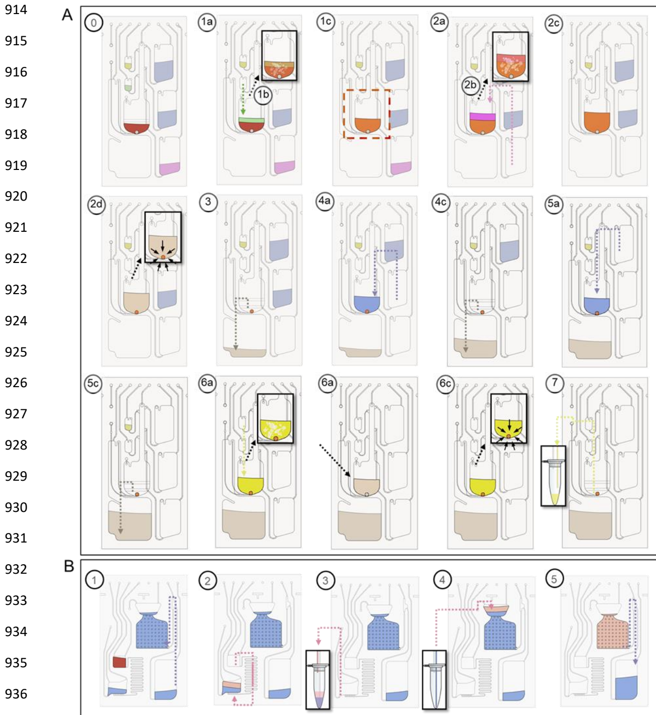
Supplemental Figure S5. Microfluidic implementation. (A) RNA extraction and (B) ddPCR assays. The platform executes a predetermined sequence of spinning and pneumatic actuation steps to perform the entire analytical protocol in an automated fashion on the cartridge. These steps are represented by the sequence of schematic images showing the status of the cartridge at different steps during the automated RNA extraction protocol and subsequent ddPCR (see text and Table S2 and Table S3 for details). The arrows point in the direction of fluid flow for each step. The activated ports at each step are highlighted by green and red circles, representing the application of positive and negative pressures at that port, respectively.
