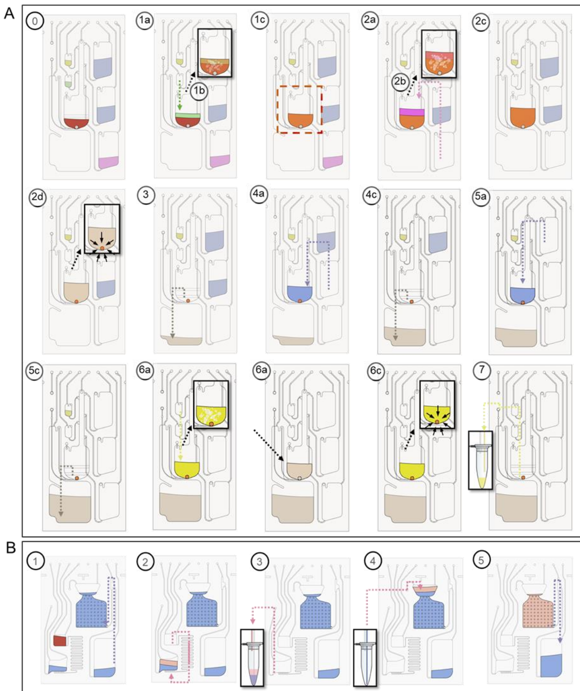
Supplemental Figure S5. Microfluidic implementation. (A) RNA extraction and (B) ddPCR assays. The platform executes a predetermined sequence of spinning and pneumatic actuation steps to perform the entire analytical protocol in an automated fashion on the cartridge. These steps are represented by the sequence of schematic images showing the status of the cartridge at different steps during the automated RNA extraction protocol and subsequent ddPCR (see text and Table S2 and Table S3 for details). The arrows point in the direction of fluid flow for each step. The activated ports at each step are highlighted by green and red circles, representing the application of positive and negative pressures at that port, respectively.
