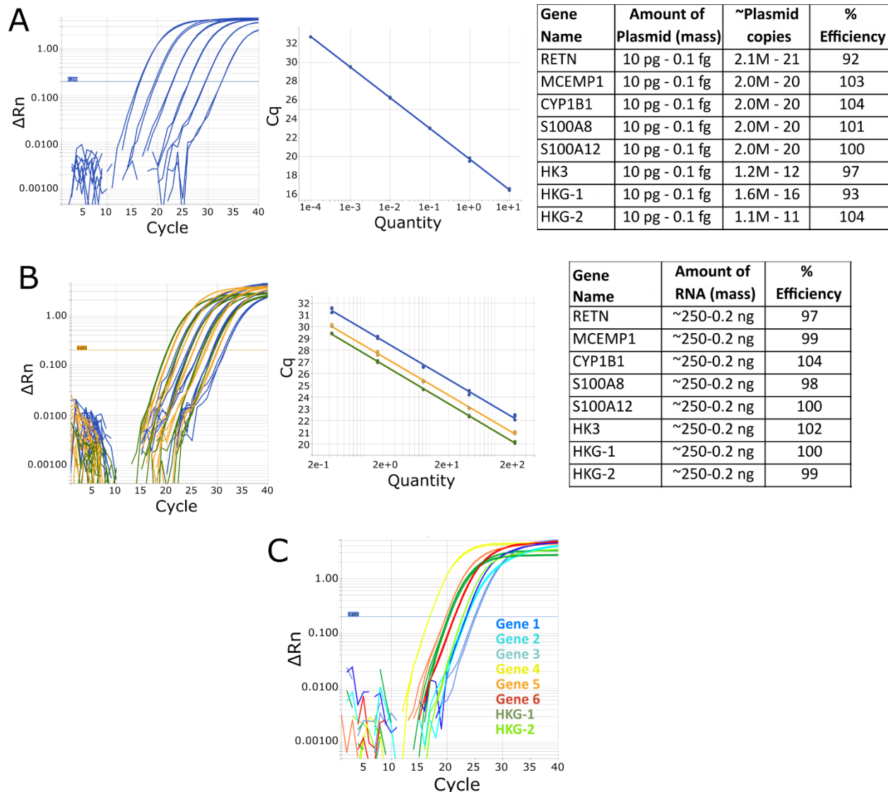
Supplemental Figure S3 – Development and performance summary of RT-qPCR primers and probes used in the Sepset signature. PCR primers were developed for each sepsis gene signature gene as well as two HKGs and their reaction efficiency was evaluated in a single-plex reaction using gene specific plasmids as the reaction template (A). Shown is the representative amplification curves and corresponding standard curve for the MCCEMP1 target along with a table summarizing the reaction efficiencies across all genes. In all cases, the efficiency was close to 100% and consistent RT-qPCR results could be obtained with as low as 10-20 copies of template in the reaction. The PCR primers were then combined in triplex reactions (B) and their reaction efficiencies were determined using RNA isolated from healthy donor blood (n=4 replicates). Shown is a representative amplification curve and corresponding standard curve for one of the multiplex reaction wells. Reaction efficiencies for all the RT-qPCR reactions were close to 100% and consistent results could be obtained with as little as ~0.2 ng of RNA used as input for the RT-qPCR reaction. A representative amplification curve for the RT-qPCR assay showing the expression pattern of all six signature genes as well as the two housekeeping genes is also shown (C).
