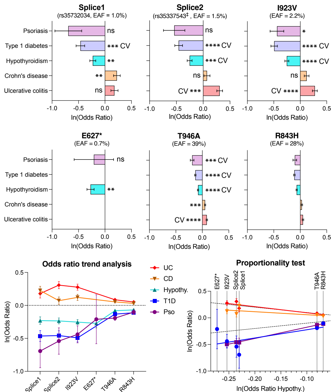
264 265 Figure 2. GWAS meta-analysis of loss-of-function MDA5 variants. (a) Effect sizes expressed in terms 266 of the odd ratio for selected MDA5 loss-of-function variants. ‡ Because rs35337543 was only available in 267 two GWAS datasets, rs72871627 ( r^2 = 0.973 ) was used as a tag for rs35337543. EAF, effect allele 268 frequency. Error bars, SEM. ns, P > 0.05 ; *, P < 0.05 ; **, P < 0.01 ; ***, P < 0.001 ; ****, P < 5 \times 10^{-8} 269 (genome-wide significance), where P is the Bonferroni-adjusted P value from marginal association 270 analysis. CV, likely causal variant present in a credible set in fine-mapping analysis. R843H was included 271 in fine-mapping analysis but excluded from marginal association analysis. See Table 1. (b) Odds ratio 272 plot for variants and diseases in (a). (c) Estimated effect sizes in hypothyroidism compared to the other 273 diseases. Hypothyroidism was selected because it was the largest dataset for which all SNPs were 274 available. Dashed lines, identity and negative identity lines. 275
