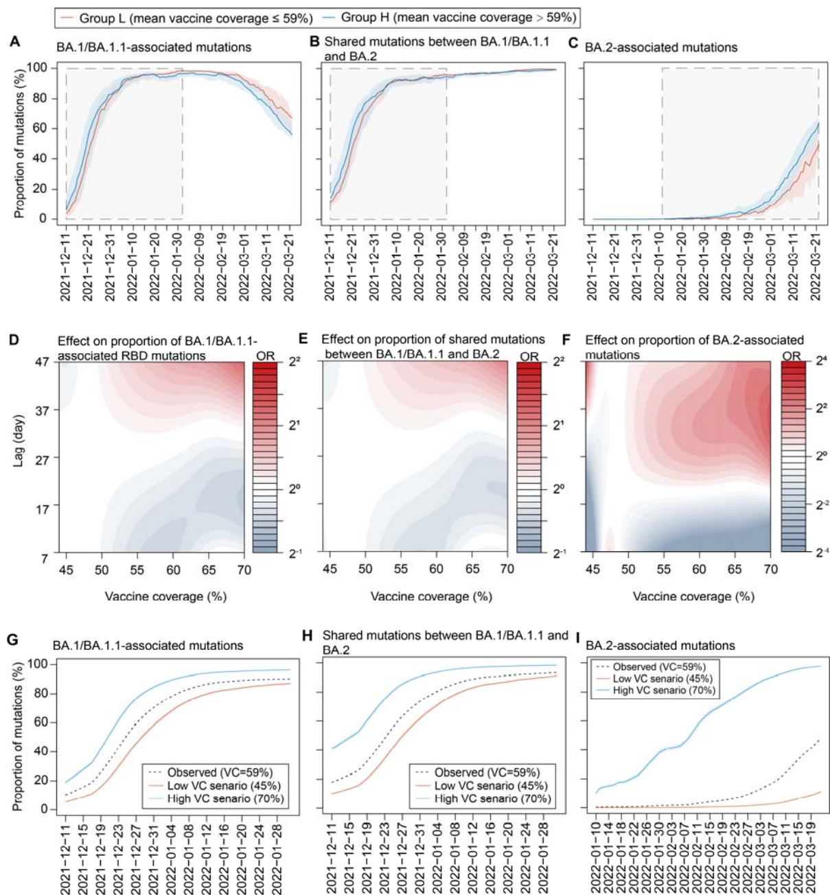
497 Figure 4 Estimated effects of vaccination coverage on the transmission of Omicron 498 mutations from the intermediate models. (A-C) Mean proportion of BA.1/BA.1.1- 499 associated mutations, shared mutations between BA.1/BA.1.1 and BA.2 subvariants, and 500 BA.2-associated mutations in Group L (with low vaccination coverage) and Group H (with 501 high vaccination coverage) states. The grey-shaded areas represented the period during which 502 the proportion of the mutation grew. The mean proportion of BA.1 associated mutations is 503 the average daily proportion of S371L, G496S, and G446S; mean proportion of BA.2- 504 associated mutations is the average daily proportion of S371F, T376A, R408S, and D405N;
