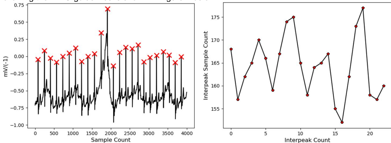
Figure 2: ECG data inverted on y axis with peak_detect(left) and interpeak array by sample count (right)
