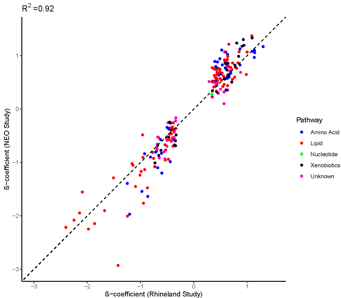
Figure S1: Correlation between the GWAS meta-analysis independent SNP ( r^2 < 0.6 )-metabolite effect sizes from the Rhineland Study and the NEO Study
