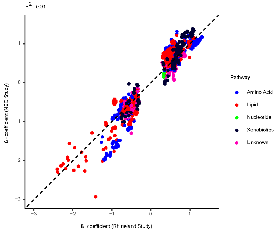
Extended Data Fig. 1 Correlation between the GWAS meta-analysis loci-metabolite effect sizes from the Rhineland Study and the NEO Study
