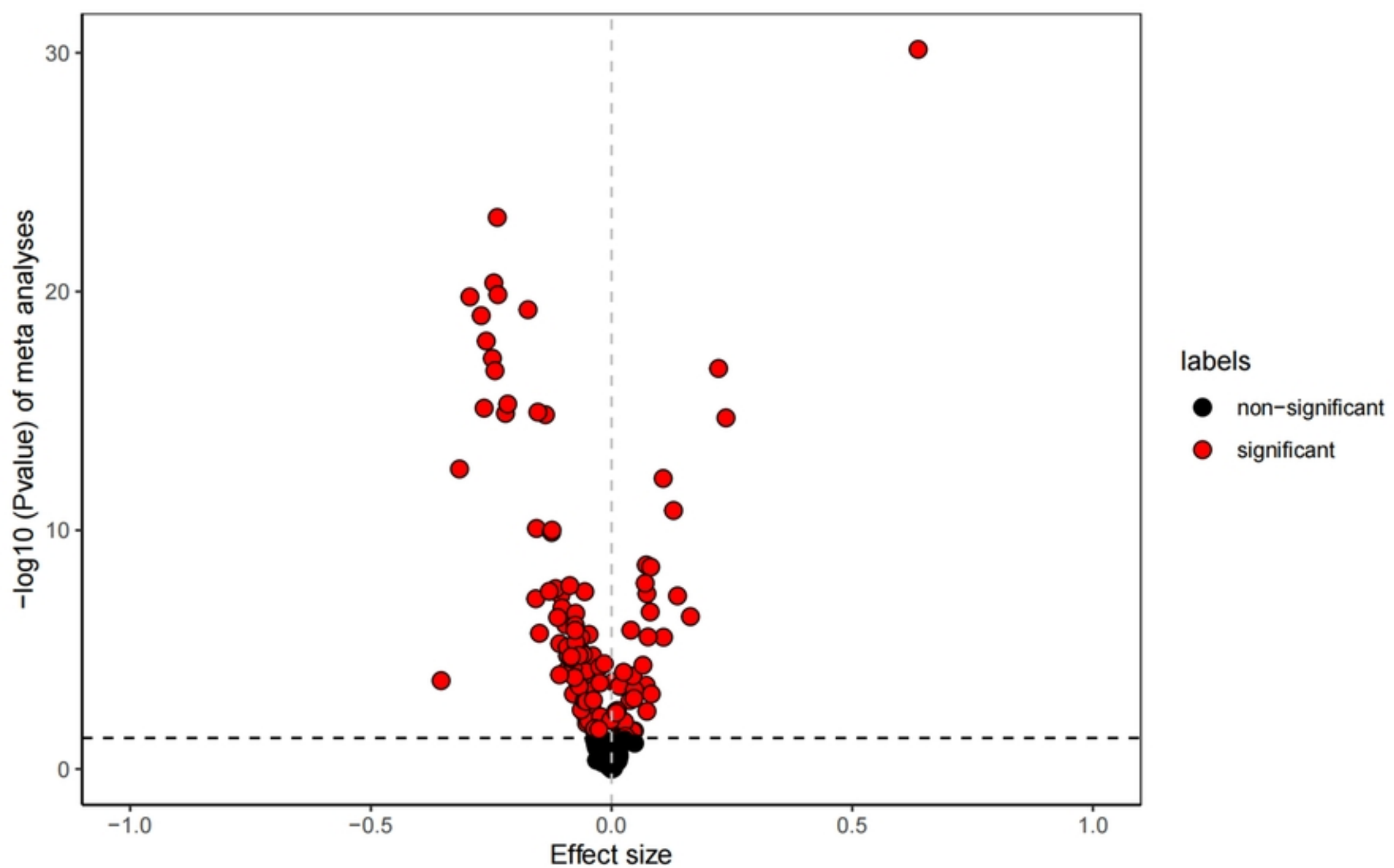
Fig 2. Volcano plot of differentially expressed genes related to m
