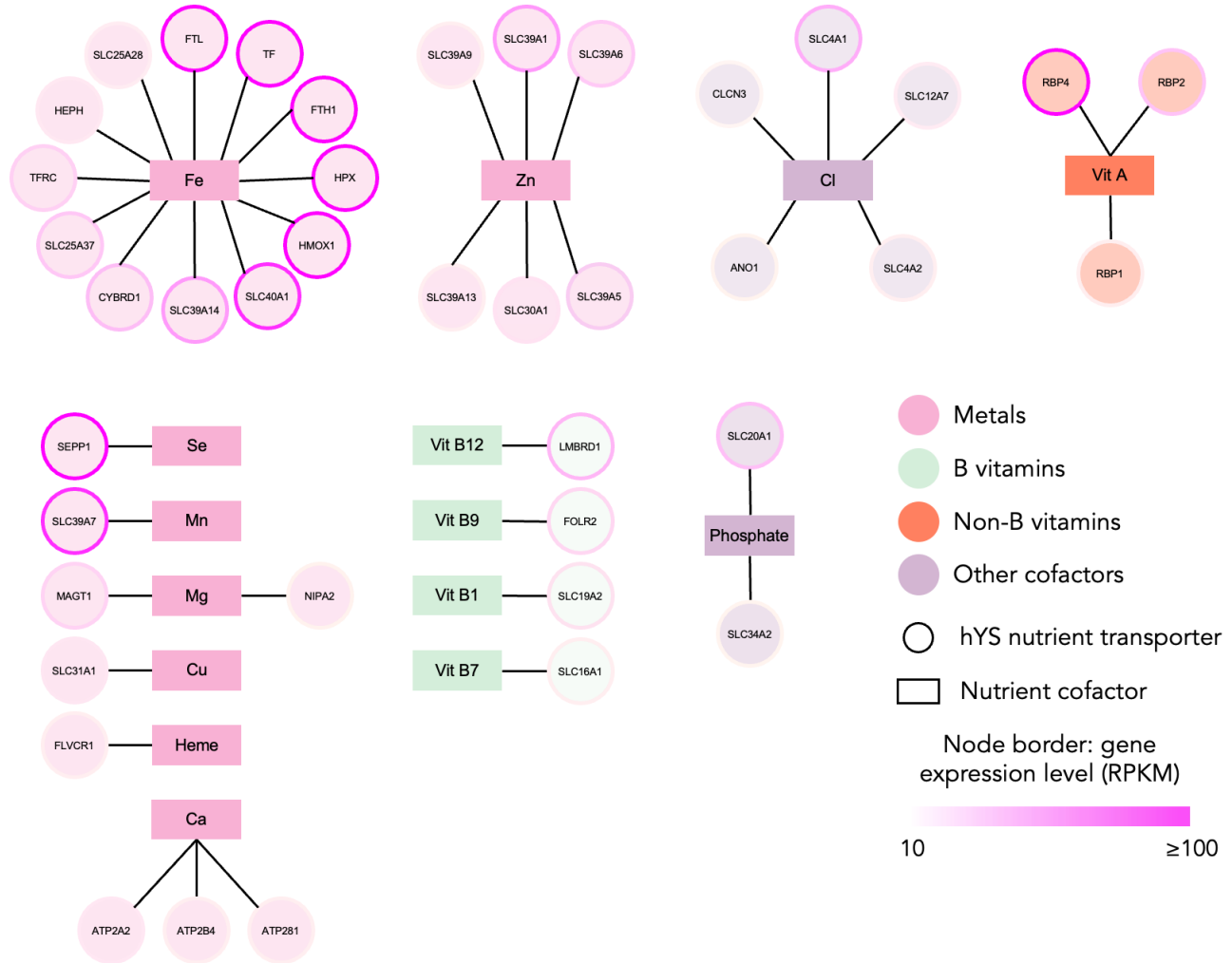
Figure 6. Highly expressed hYS genes encoding for nutrient transporters. hYS nutrient transporters (circle nodes) connected to the nutrient that they transport (rectangle nodes) via lines (edges). Node border colour = gene expression in RPKM (reads per kilobase of transcript), per million mapped reads. Fe = iron; Zn = zinc; Cl = chloride; Mg; magnesium; Mn = manganese; Cu = copper; Se = selenium; Ca = calcium.
