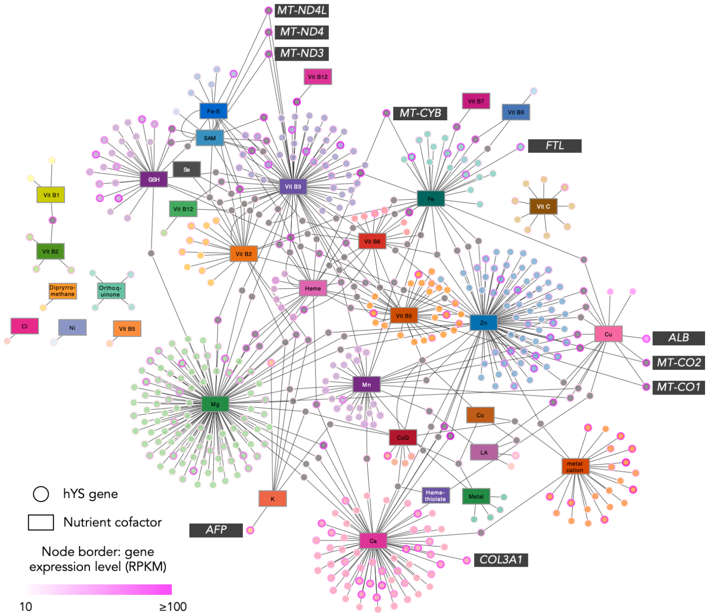
Figure 2. Nutrient-gene interactions in hYS. Nutrient-sensitive genes (circle nodes) connected to their nutrient cofactors (rectangular nodes) via edges (lines). Genes with one nutrient cofactor are colour-coordinated to their respective cofactor. Genes (nodes) with >1 nutrient cofactor are grey. The top 10 most highly expressed hYS are labelled. MT-ND4L = Mitochondrially Encoded NADH Dehydrogenase 4L; MT-ND3/4 = Mitochondrially Encoded NADH; FTL = Ferritin Light Chain; MT-CYB = Mitochondrially Encoded Cytochrome B; MT-CO1 = Mitochondrially Encoded Cytochrome C Oxidase; ALB = Albumin; MT-CO2 = Mitochondrially Encoded Cytochrome C Oxidase II; COL3A1 = Collagen Type III Alpha 1 Chain; AFP = Alpha Fetoprotein; RPKM = reads per kilobase of transcript, per million mapped reads. Vit = Vitamin; CoQ = ubiquinone.
