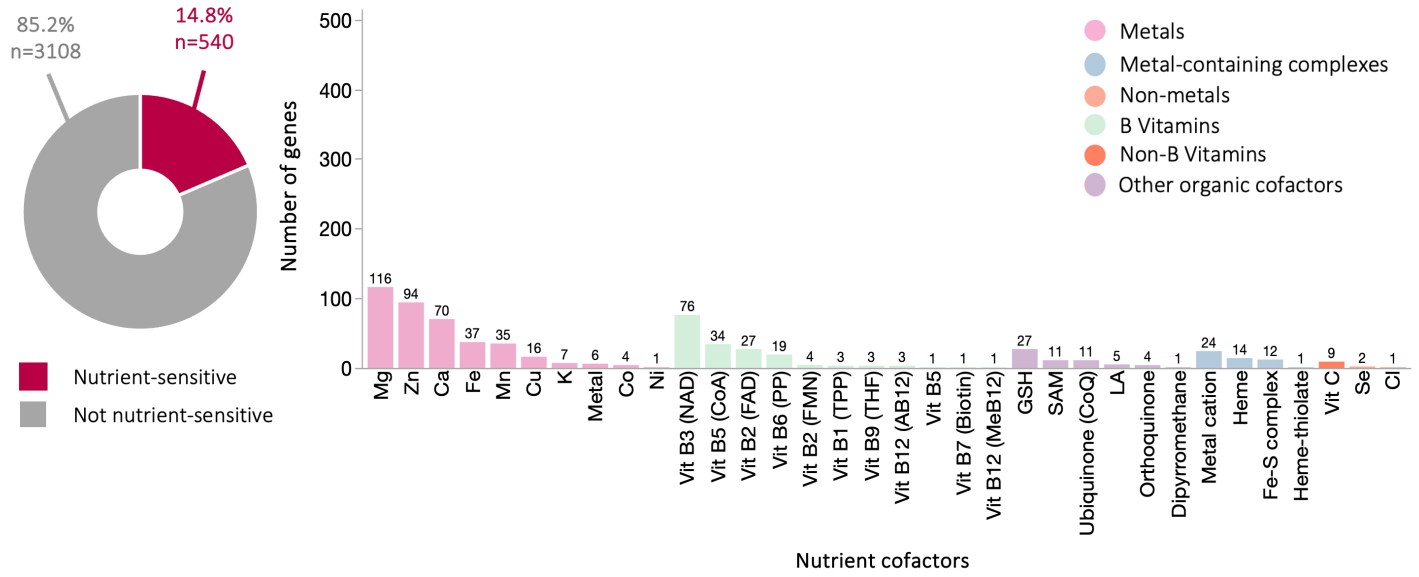
Figure 1. Highly expressed nutrient-sensitive genes in hYS genes (n=3648). Proportion of hYS genes that are nutrient-sensitive (left column; donut charts) to the nutrients indicated in the histograms (right column; bar charts). Numbers above the histogram bars = total number of genes sensitive to that nutrient. RPKM = Reads per kilobase of transcript, per million mapped reads; SAM = S-Adenosyl methionine; GSH = glutathione; Mo = molybdenum; MPT = molybdopterin.
