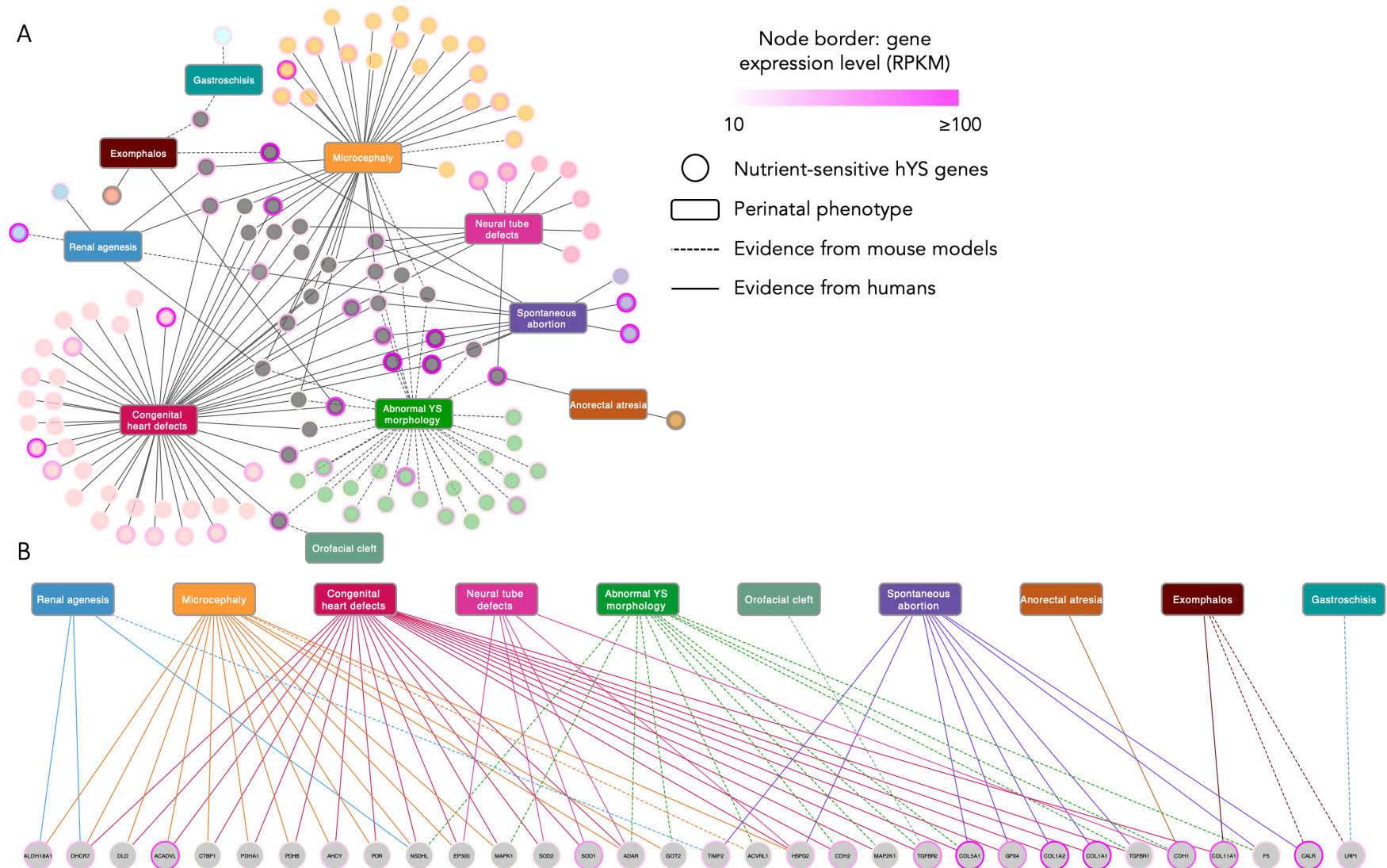
Figure 7. Adverse perinatal phenotypes with embryonic origins associate with highly expressed nutrient-sensitive hYS genes. (A) Connections between adverse perinatal phenotypes of embryonic origin and highly expressed nutrient-sensitive hYS genes (circle nodes; n=117 ). (B) Highly expressed hYS genes associated with >1 adverse perinatal phenotype. Genes are colour in coordination with associated phenotypes. Genes associated with >1 phenotype are grey ( n=32 ). Dotted edges = mouse disease association. Full edges = human disease association. Node border colour = gene expression in RPKM (reads per kilobase of transcript), per million mapped reads.
