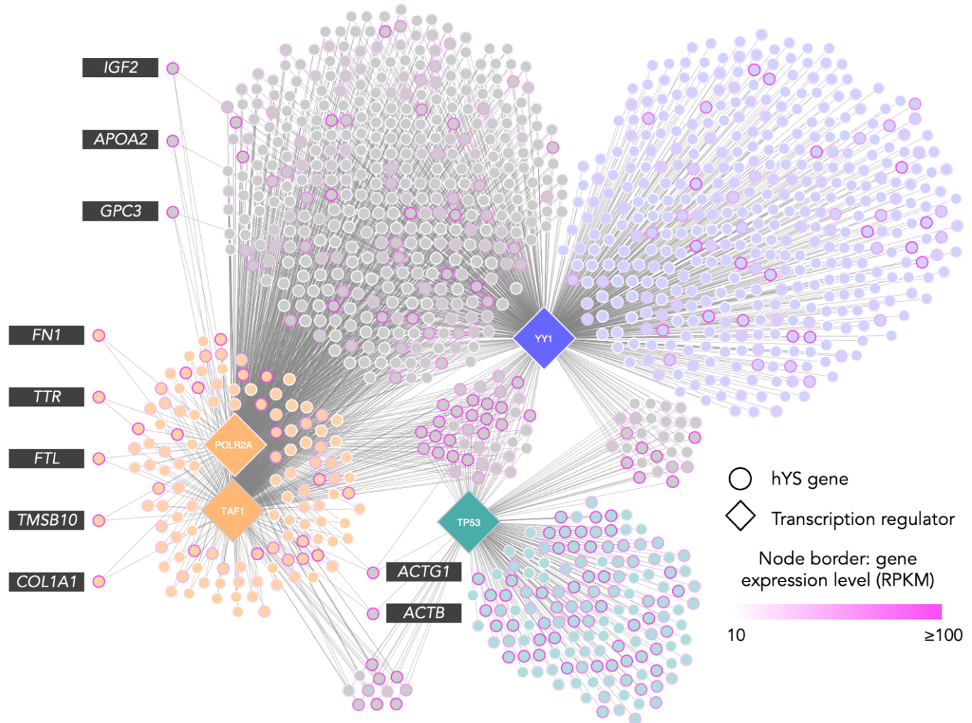
Figure 5. Nutrient-sensitive transcription regulators of hYS genes. Nutrient-sensitive transcription regulators (diamond nodes; n=4) connected to hYS gene targets (circle nodes; n=1127). Node border colour = gene expression in RPKM (reads per kilobase of transcript), per million mapped reads. The top 10 most highly expressed hYS gene targets are labelled. ACTB = Actin Beta; ACTG1 = Actin Gamma 1; APOA2 = Apolipoprotein A2; COL1A1 = Collagen Type I Alpha 1; FN1 = Fibronectin 1; FTL = Ferritin Light Chain; GPC3 = Glypican 3; IGF2 = Insulin Like Growth Factor 2; TMSB10 = Thymosin Beta 10; TTR = Transthyretin.
