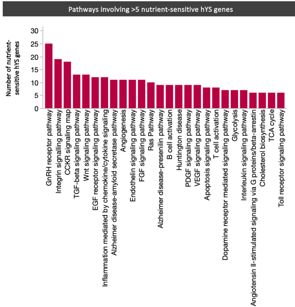
Figure 4. PANTHER pathways involving >5 nutrient-sensitive hYS genes. GnRH = gonadotropin-releasing hormone; TGF = Transforming growth factor; EGF = Epidermal growth factor; FGF = Fibroblast growth factor; VEGF = Vascular endothelial growth factor; PDGF = Platelet derived growth factor.
