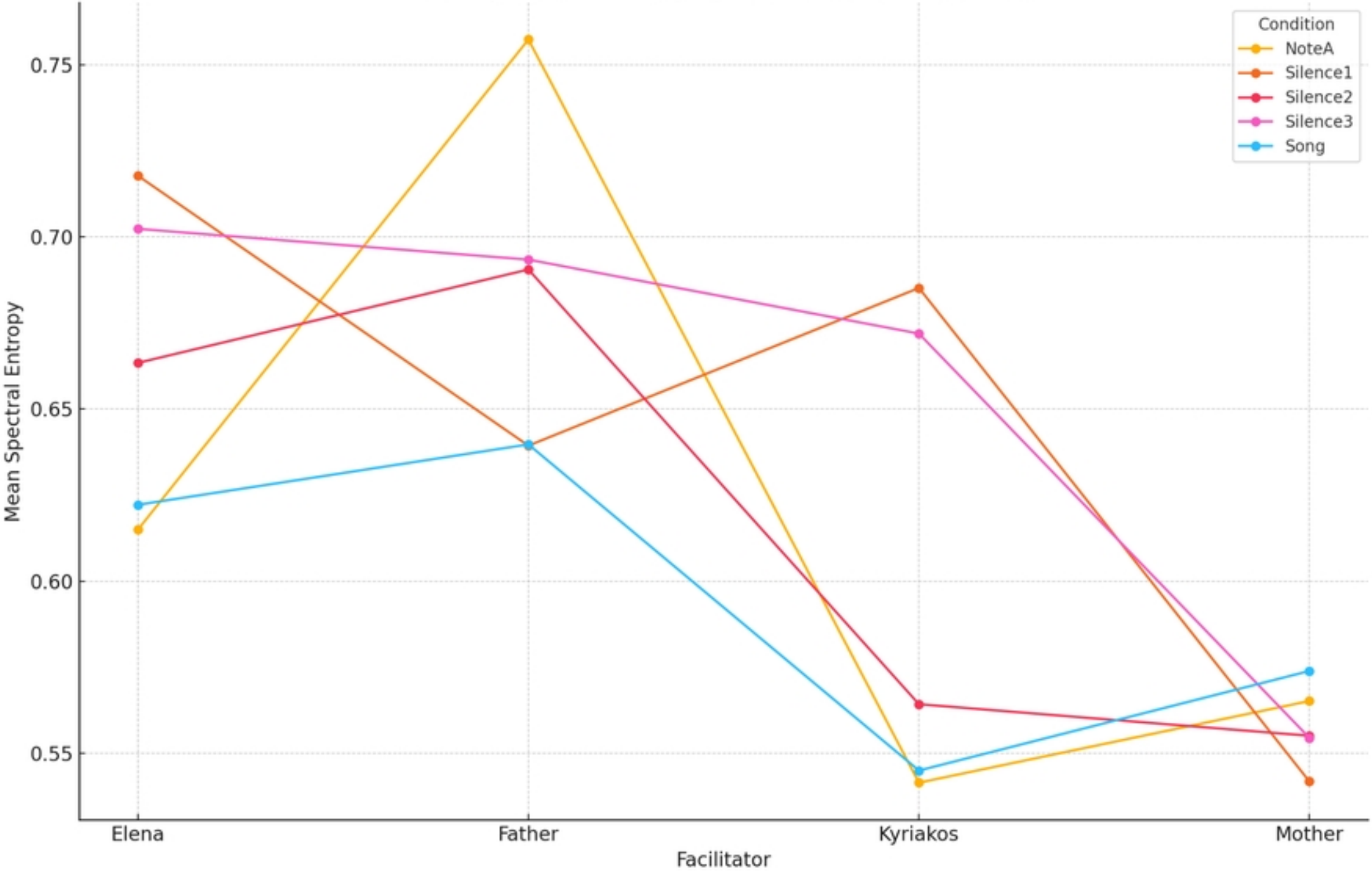
Mean Spectral Entropy by Facilitator and Condition
