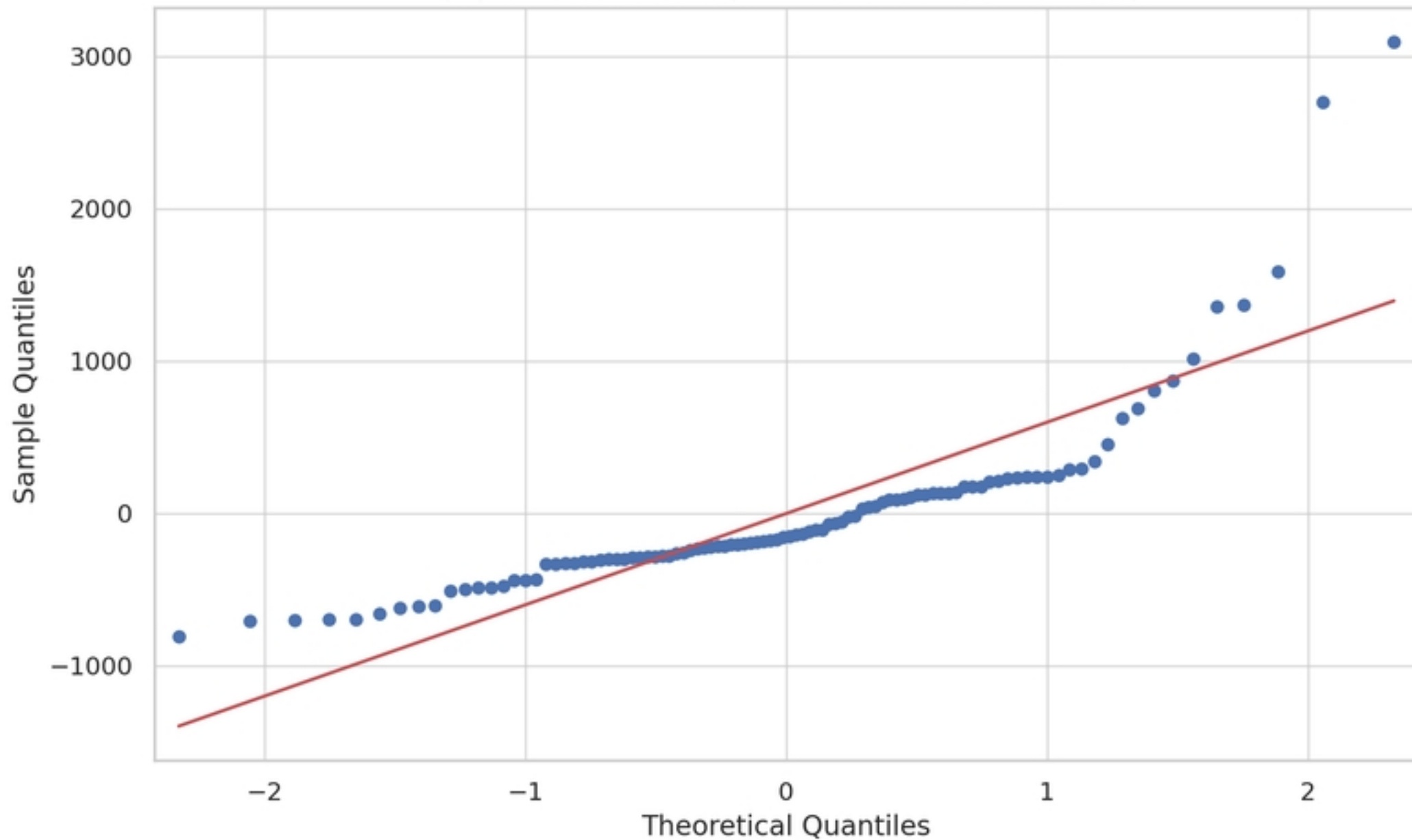
Q-Q Plot of Residuals (Reference: Elena & Silence 1)
