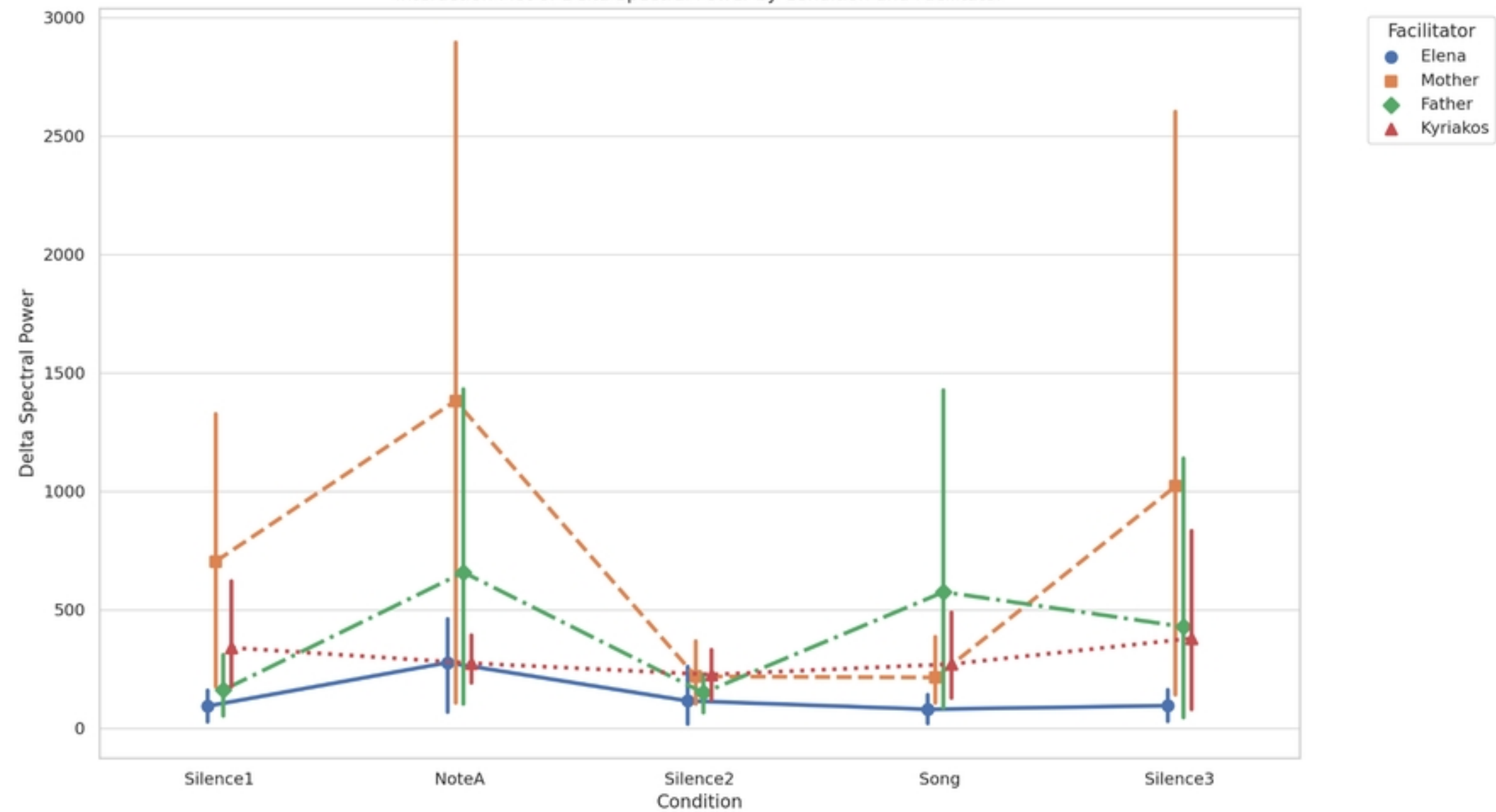
Interaction Plot of Delta Spectral Power by Condition and Facilitator
