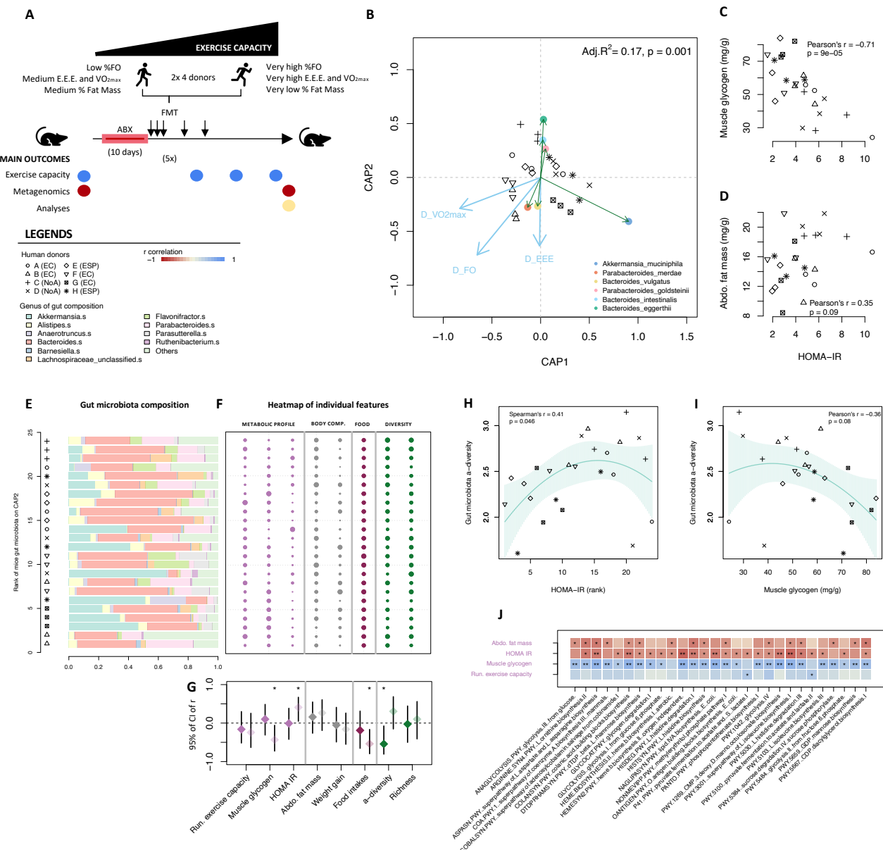
426 Figure 3. The gut bacterial ecosystem from human donors affects insulin sensitivity and muscle 427 glycogen stores in transfected mice, depending on the donor's exercise capacity. (A) Experimental 428 design of FMT from human donors with heterogeneous exercise capacity into antibiotic-pretreated 429 mice. (B) Canonical Analysis of Principal Coordinates (CAP) between the Principal Coordinates of the 430 pairwise dissimilarity matrix (Bray Curtis) of mice's gut microbiota compositions and the donors' 431 exercise capacity parameters (blue arrows). The points represent the most associated species of the 432 second axis of the CAP. (C) Muscle glycogen content according to HOMA-IR. (D) Abdominal fat mass 433 according to HOMA-IR. (E) Ranked mice from the CAP2 with the corresponding gut microbiota 434 composition (1 line = 1 mice). (F) Heatmap of metabolic profile, body composition, food intake and gut 435 microbiota composition's diversities (1 line = 1 mice), the width of each point is normalized by the 436 intra-variable maximum. (G) 95% confidence interval of the r correlation between each variable either
