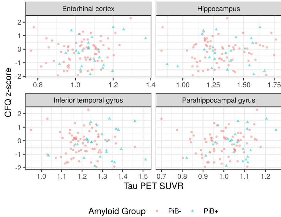
Figure 3: CFQ score at index visit versus regional tau SUVR.
