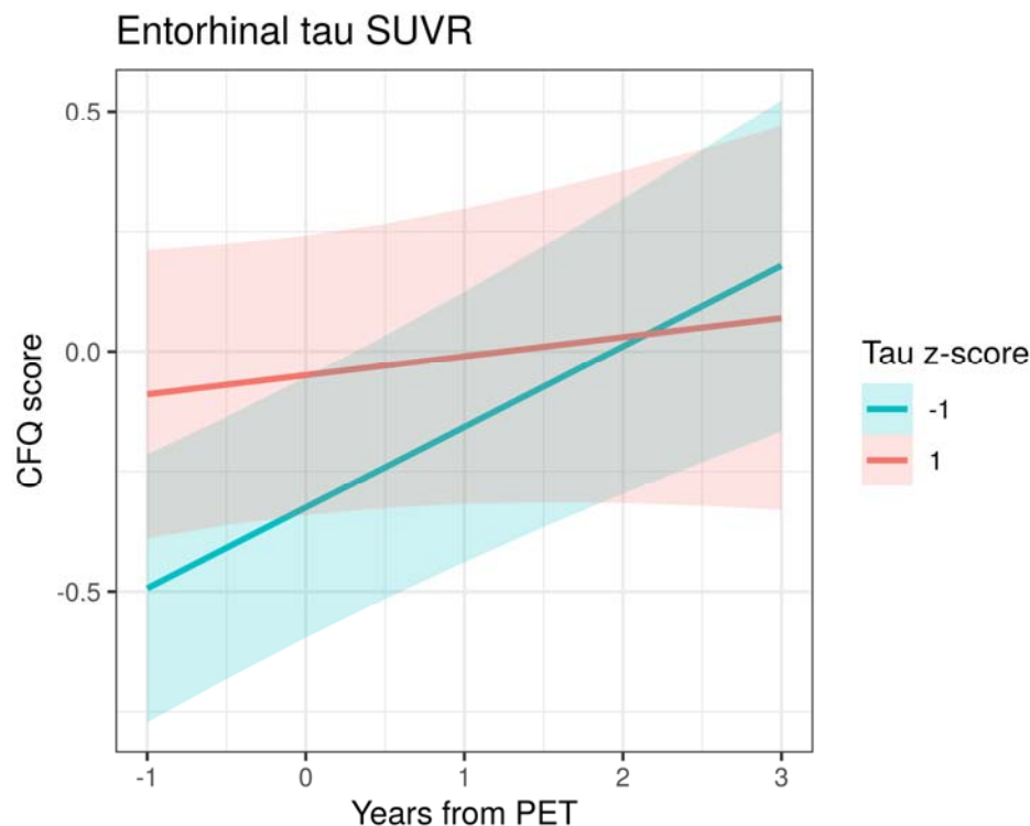
Figure 2: Longitudinal CFQ trajectories by entorhinal tau SUVR z-score based on linear mixed effects model estimates.
