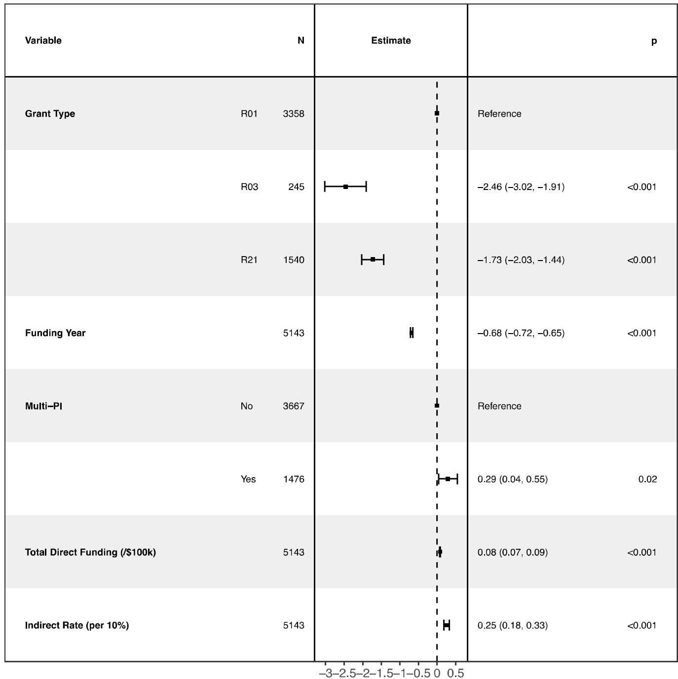
Figure 1. Multiple linear regression model of association between indirect rate and H-index at five years
