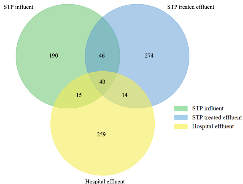
406 407 Figure 3: Venn diagram showing the shared (46, 40, 14 and 15) and exclusive (190, 274 and 408 259) antibiotic resistance genes (ARGs), including both known and novel, across the three 409 samples (hospital effluent, sewage treatment plant (STP) influent and STP treated effluent).
