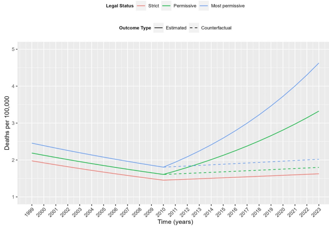
Difference in difference estimation for deaths per 100,000
