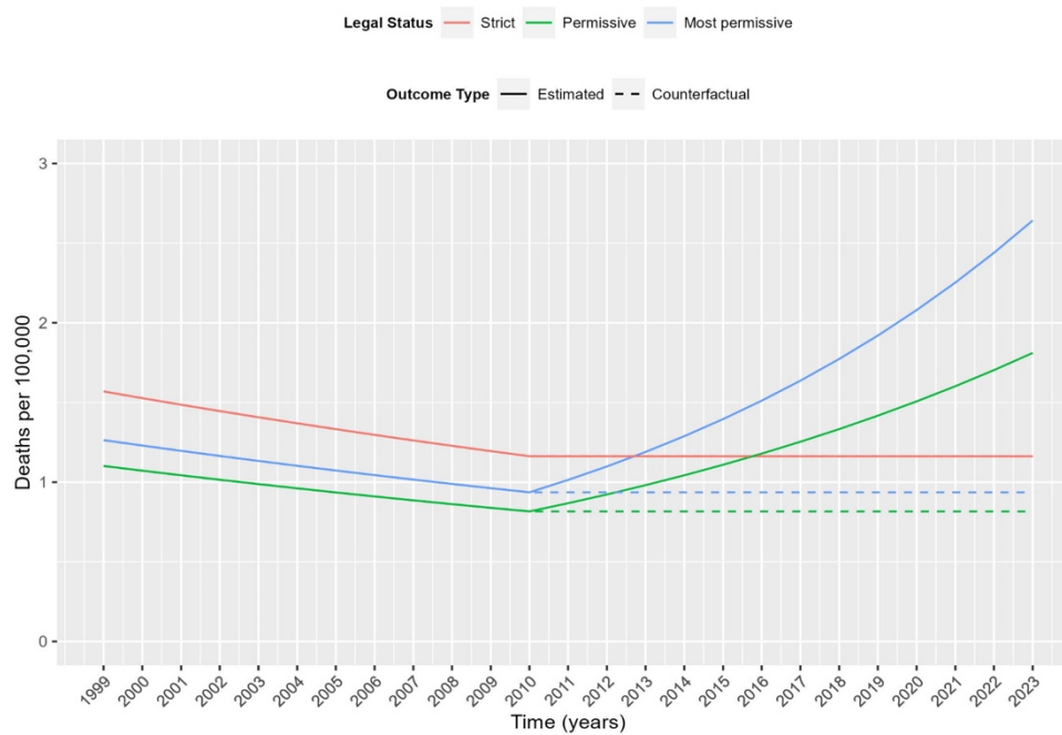
DiD estimation for deaths per 100,000 - Homicide
