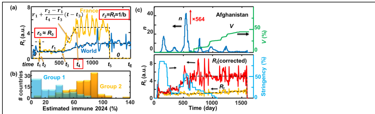
Figure 6. (a) Example fitting of R_t curve using the laydown ‘5’ shape for France and world average. (b) Histogram of Group 1 countries that do not follow (a) and Group 2 countries that follow the laydown ‘5’ pattern in (a) with today’s immune ratios. (c) Example data treatment of Group 1 countries with low COVID-19 testing rates, briefly, multiplying a testing rate correction factor estimated using world average timing and recalculating the R_t values.
