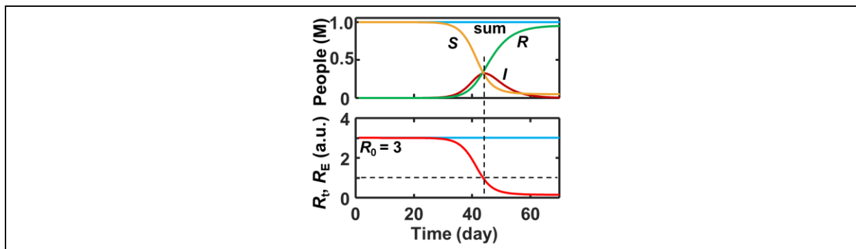
Figure 2. Simulation of SIR model with R_t = R_0 = 3.0 . Detail algorithm available in the literature and an Excel file running the simulation can be found in our previous publications. 12,22,23
