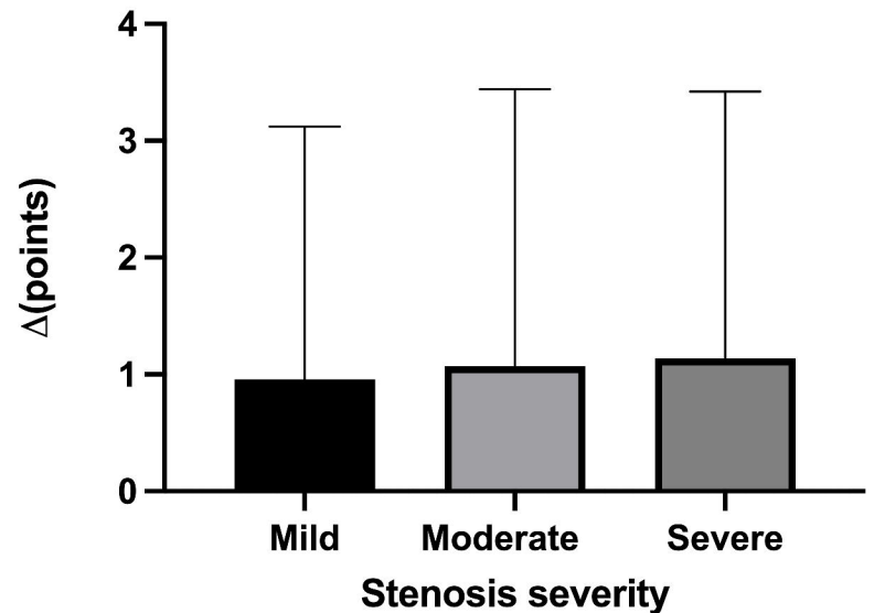
PSFS improvement
