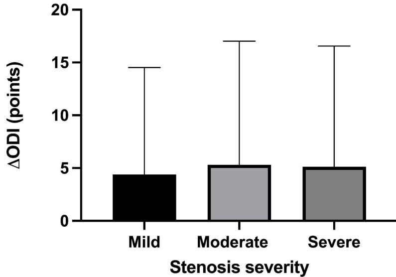
ODI improvement
