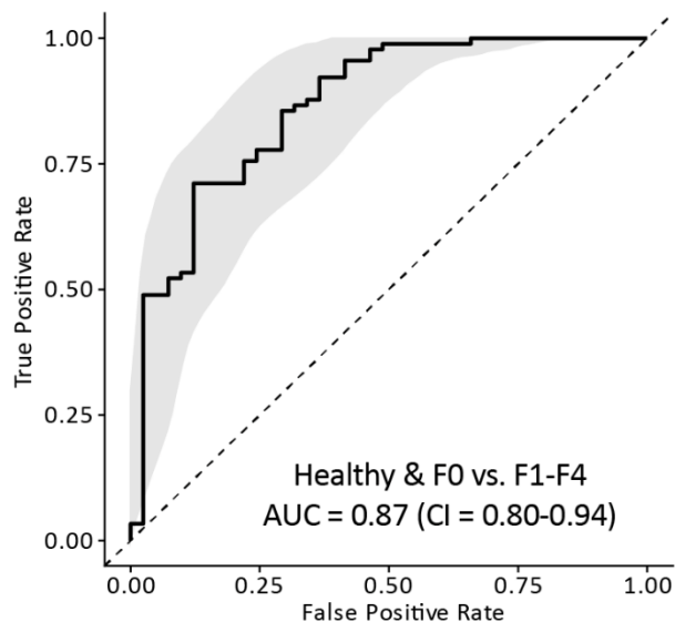
Figure 4. ROC analysis and associated AUC value for the single predictor model including A4L, illustrating its power to predict fibrosis
