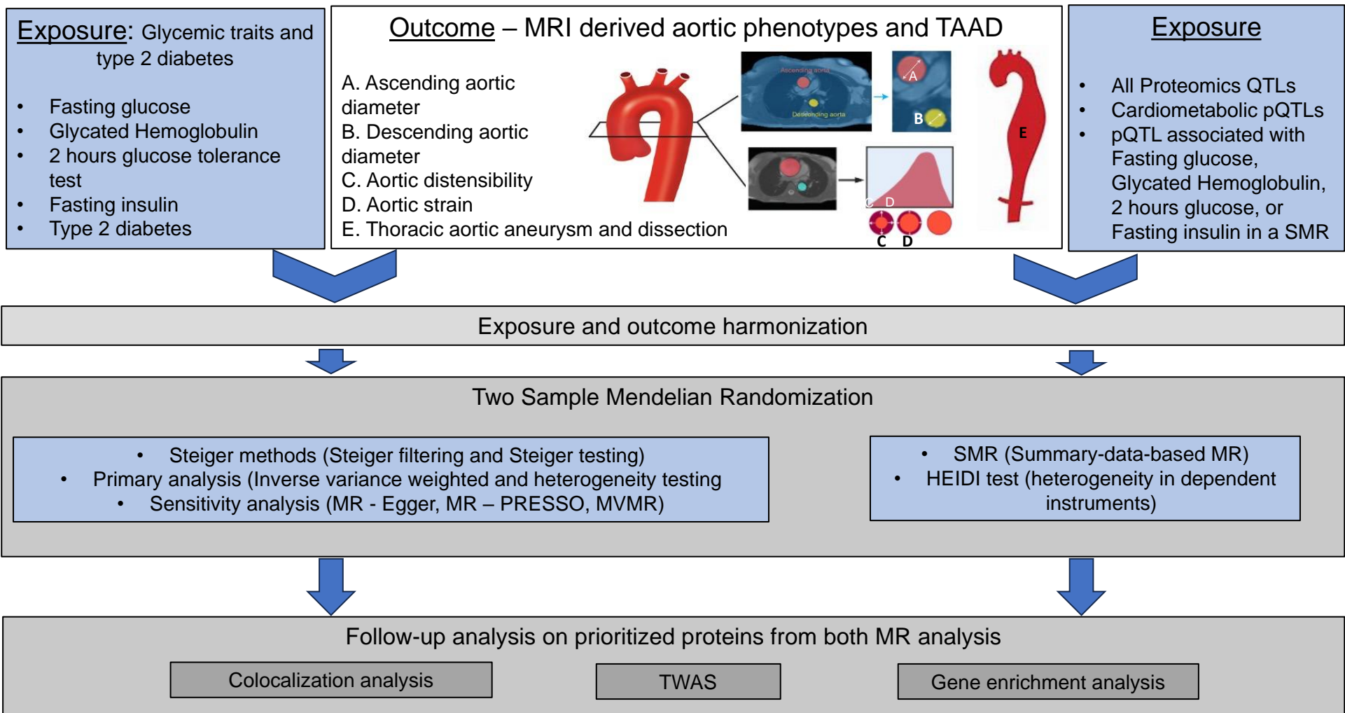
Figure 1: Flowchart Mendelian Randomization analysis investigating the causal association between glycaemic traits and aortic measurement and diseases. Sample size description for each summary statistic is presented in the table S2.
