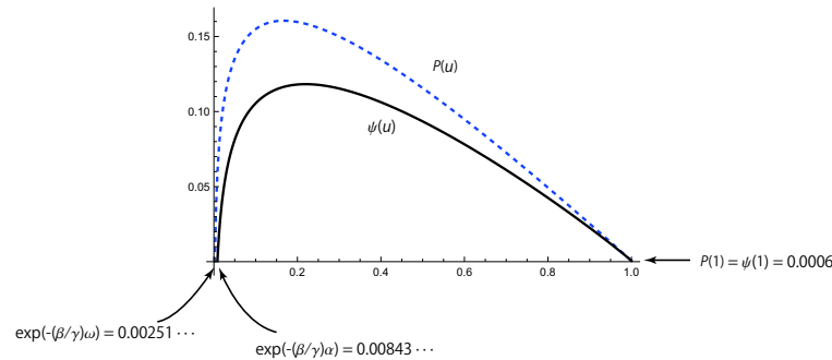
Figure 4: Variations of P(u) = \beta N - \beta\tilde{S}e^{(\beta/\gamma)\tilde{R}}u + \gamma \log u (dashed curve) and \psi(u) (solid curve) obtained by the numerical integration of the initial value problem (58)–(60) for N = 1000, \tilde{S} = 998, \tilde{I} = 2, \tilde{R} = \tilde{V} = 0, \beta = 0.3/1000, \gamma = 0.05 and \sigma = 0.008 . In this case we get \alpha = 795.93 \dots, e^{-(\beta/\gamma)\alpha} = 0.00843 \dots, \omega = 997.48 \dots, e^{-(\beta/\gamma)\omega} = 0.00251 \dots, P(1) = \beta N - \beta\tilde{S} = 0.0006 and \psi(1) = \beta\tilde{I} = 0.0006 . Moreover, P(e^{-(\beta/\gamma)\omega}) = 0 and \lim_{u \rightarrow e^{-(\beta/\gamma)\alpha}+0} \psi(u) = 0 .
