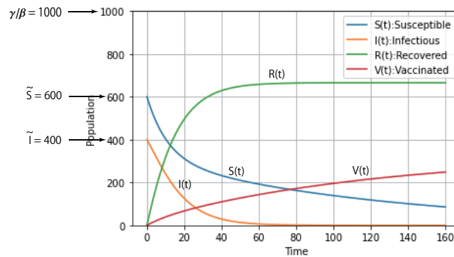
Figure 6: Variations of S(t), V(t), I(t) and R(t) obtained by the numerical integration of the initial value problem (1)–(5) for N = 1000, \tilde{S} = 600, \tilde{I} = 400, \tilde{R} = \tilde{V} = 0, \beta = 0.1/1000, \gamma = 0.1 and \sigma = 0.008 . In this case we find that \tilde{S}(= 600) < (\gamma/\beta)(= 1000) , I(t) is decreasing on [0, \infty) and I(\infty) = 0 .
