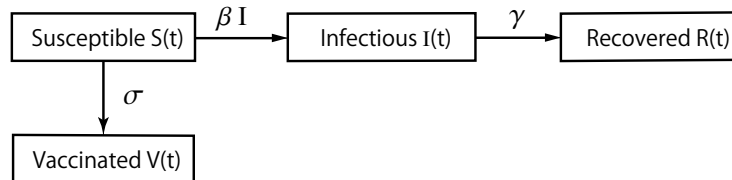
Figure 1: Flow diagram of the SVIR epidemic model.
