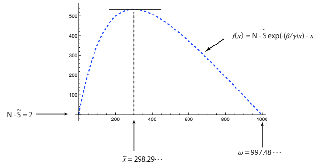
Figure 2: Variation of f(x) = N - \tilde{V} - \tilde{S}e^{(\beta/\gamma)\tilde{R}}e^{-(\beta/\gamma)x} - x = N - \tilde{S}e^{-(\beta/\gamma)x} - x for N = 1000, \tilde{S} = 998, \tilde{R} = \tilde{V} = 0, \beta = 0.3/1000, \gamma = 0.05 . In this case we find that N - \tilde{S} = 2, \tilde{x} = (500/3) \log((3/500) \times 998) = 298.29\dots and \tilde{R}(=0) < \omega = 997.48\dots < N - \tilde{V}(=1000) .
