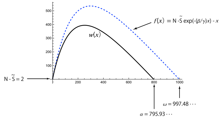
Figure 3: Variations of f(x) (dashed curve) and w(x) (solid curve) obtained by the numerical integration of the initial value problem (46)–(48) for N = 1000 , \tilde{S} = 998 , \tilde{I} = 2 , \tilde{R} = \tilde{V} = 0 , \beta = 0.3/1000 , \gamma = 0.05 and \sigma = 0.008 . In this case we obtain \omega = 997.48 \dots , \alpha = 795.93 \dots , f(0) = N - \tilde{S} = 2 and w(0) = \tilde{I} = 2 .
