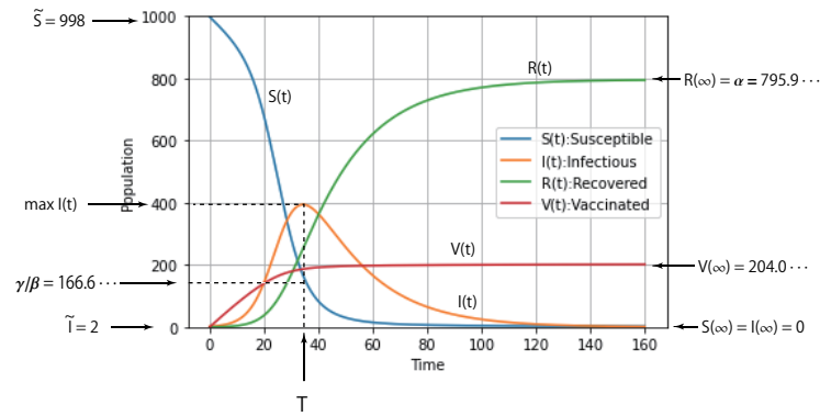
Figure 5: Variations of S(t), V(t), I(t) and R(t) obtained by the numerical integration of the initial value problem (1)–(5) for N = 1000, \tilde{S} = 998, \tilde{I} = 2, \tilde{R} = \tilde{V} = 0, \beta = 0.3/1000, \gamma = 0.05 and \sigma = 0.008 . In this case we obtain \tilde{S} (= 998) > (\gamma/\beta) (= 166.6 \dots) , R(\infty) = \alpha = 795.9 \dots , S(\infty) = I(\infty) = 0 and V(\infty) = 204.0 \dots .
