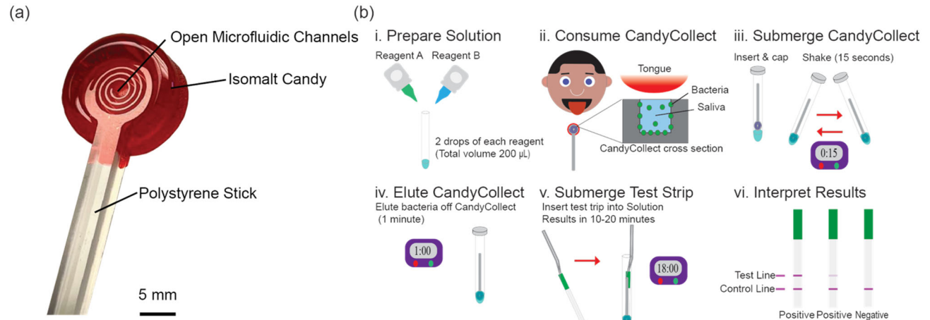
215 216 Figure 1. (a) Schematic of the CandyCollect Device. The open fluidic channels milled into the head of the plasma-treated 217 polystyrene stick allow pathogens to adhere over sampling time as the user consumes the isomalt candy. (b) Workflow to 218 incorporate sampling with the CandyCollect device with the Areta Strep A Swab Test™ protocol. (i) Elution solution is prepared 219 before sampling in the kit-provided tube by combining 100 µL (2 drops) of Reagent A (2.0 M sodium nitrite) and 100 µL (2 220 drops) of Reagent B (0.4 M acetic acid) for a total elution solution volume of 200 µL. (ii) To sample, the participant places the 221 CandyCollect device in their mouth and consumes the isomalt candy on the CandyCollect device until the candy is completely 222 dissolved. S. pyogenes collects on the plasma-treated open-fluidic channels within the CandyCollect device over time. (iii) After 223 sampling, the CandyCollect device is added to the tube of elution solution, and the tube is capped and shaken for 15 s to ensure 224 that the elution solution reaches the channels. (iv) The tube is then set aside for 1 minute. (v) The tube is then uncapped, and the 225 kit-provided test strip is dipped into the elution solution for 10 s or until the fluid visibly starts to wick on the testing section of 226 the lateral flow strip. Test results are valid for 10 to 20 min after complete wicking. (vi) The presence of a test and control line 227 indicates a positive result; a control line only indicates a negative result.
