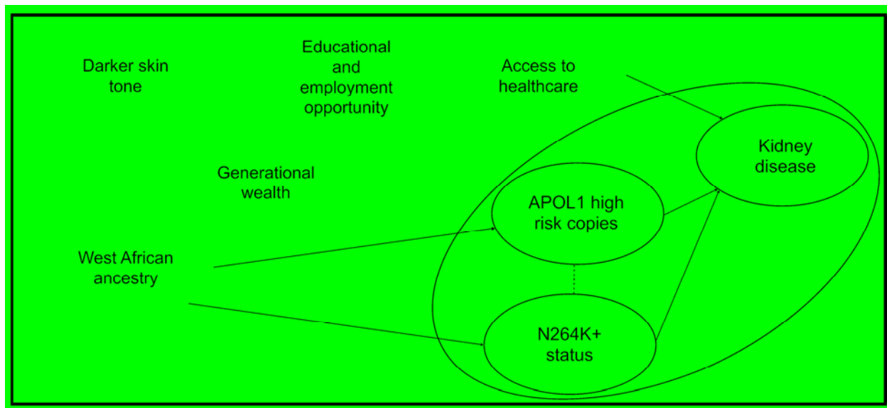
Fig 14. Causal directed acyclic graph (DAG) that the study might have imagined (with our modifications).
