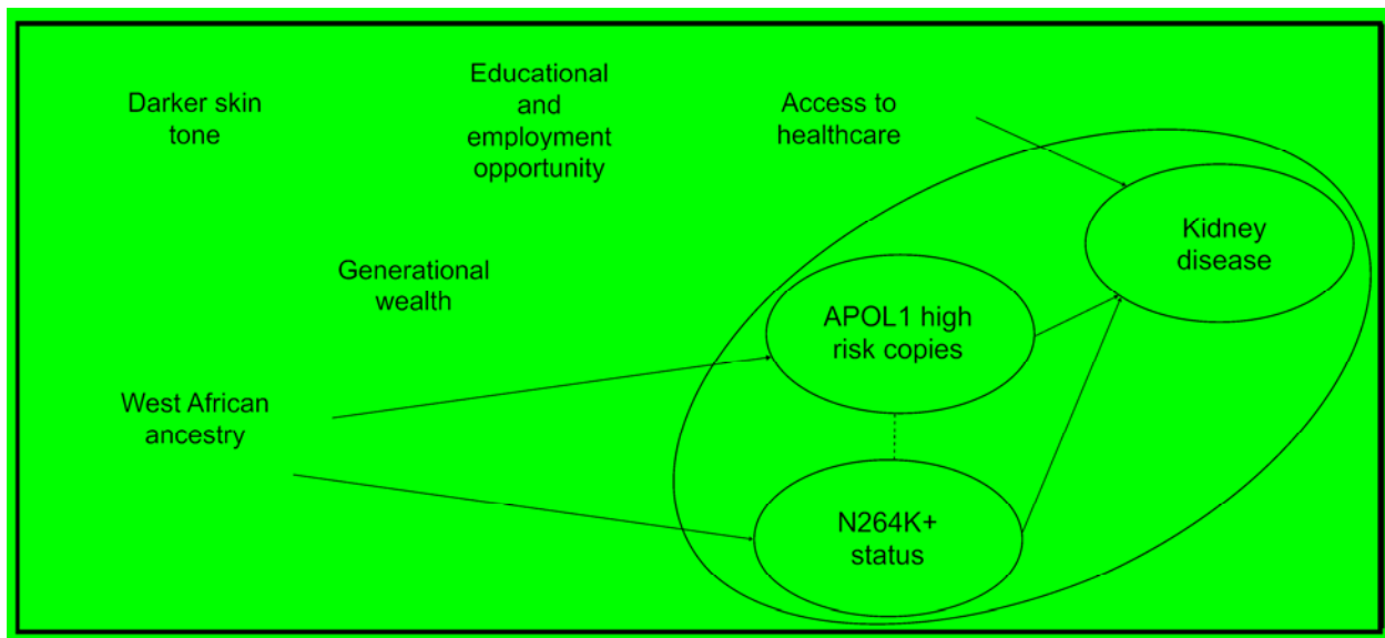
Fig 14. Causal directed acyclic graph (DAG) that the study might have imagined (with our modifications). One back door path from APOL1 to kidney disease is via West African ancestry (i.e., West African ancestry increases odds a person has APOL1 high-risk copies but also alters physical appearance, and physical appearance feeds discrimination). The study assumed the 10 ancestry principal components (plus other variables in other models) analytically controlled for this to justify focusing on relationships in the shaded area. First, we disagree that ancestry principal components controlled for the back door path via skin tone. Second, even if principal components addressed the confound of skin tone, that does not account for the history of discrimination that is its own confound, including generational wealth as a significant factor. Third, given their regional dependence and low frequencies, the inclusion of both N264K and APOL1 in one analysis is problematic. This approach leads to redundancy and collinearity, resulting in uninterpretable coefficients.
