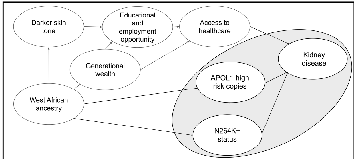
Fig 14. Causal directed acyclic graph (DAG) that the study might have imagined (with our modifications).
