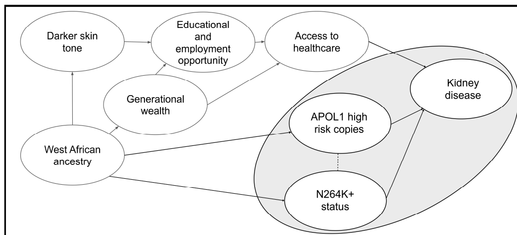
Fig 15. Causal directed acyclic graph (DAG) that the study might have imagined (with our modifications).
