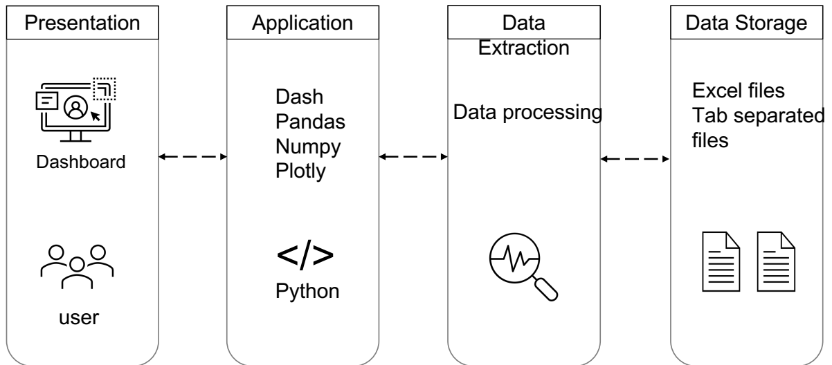
Figure 2: Illustration of the Kenya COVID-19 dashboard architecture from backend to frontend. When users select on components on the dashboard, python libraries are utilized to query and extract the dataset from stored files, generate visuals that are then displayed on the users' screen.
