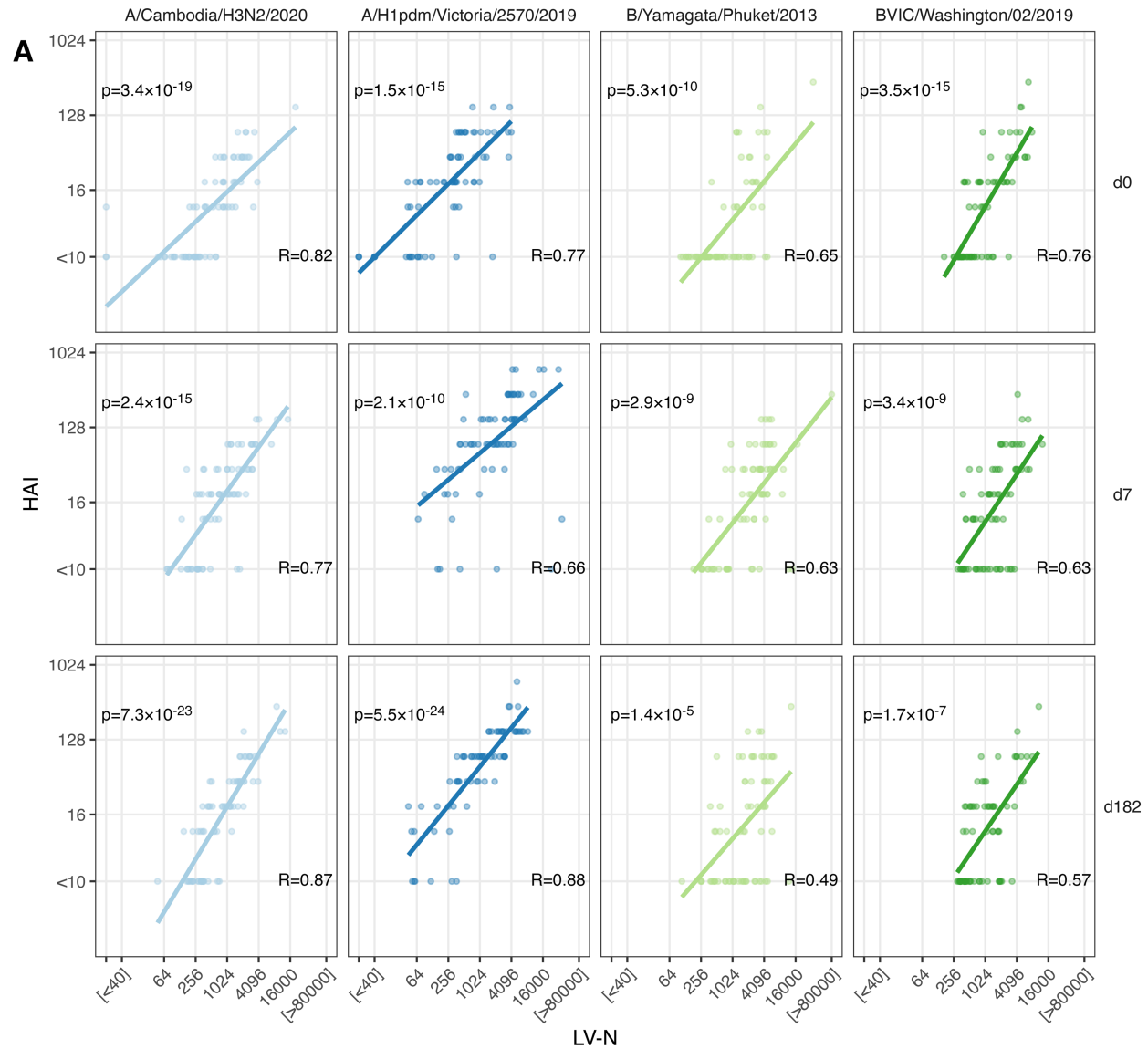
Fig 2. Comparison of haemagglutinin inhibition and high-throughput live influenza neutralisation assays (A) Correlation between HAI and LV-N for each flu virus tested, at each venepuncture. In (A), Spearman correlation coefficients and P values are shown, and a fit line from linear regression plotted.
