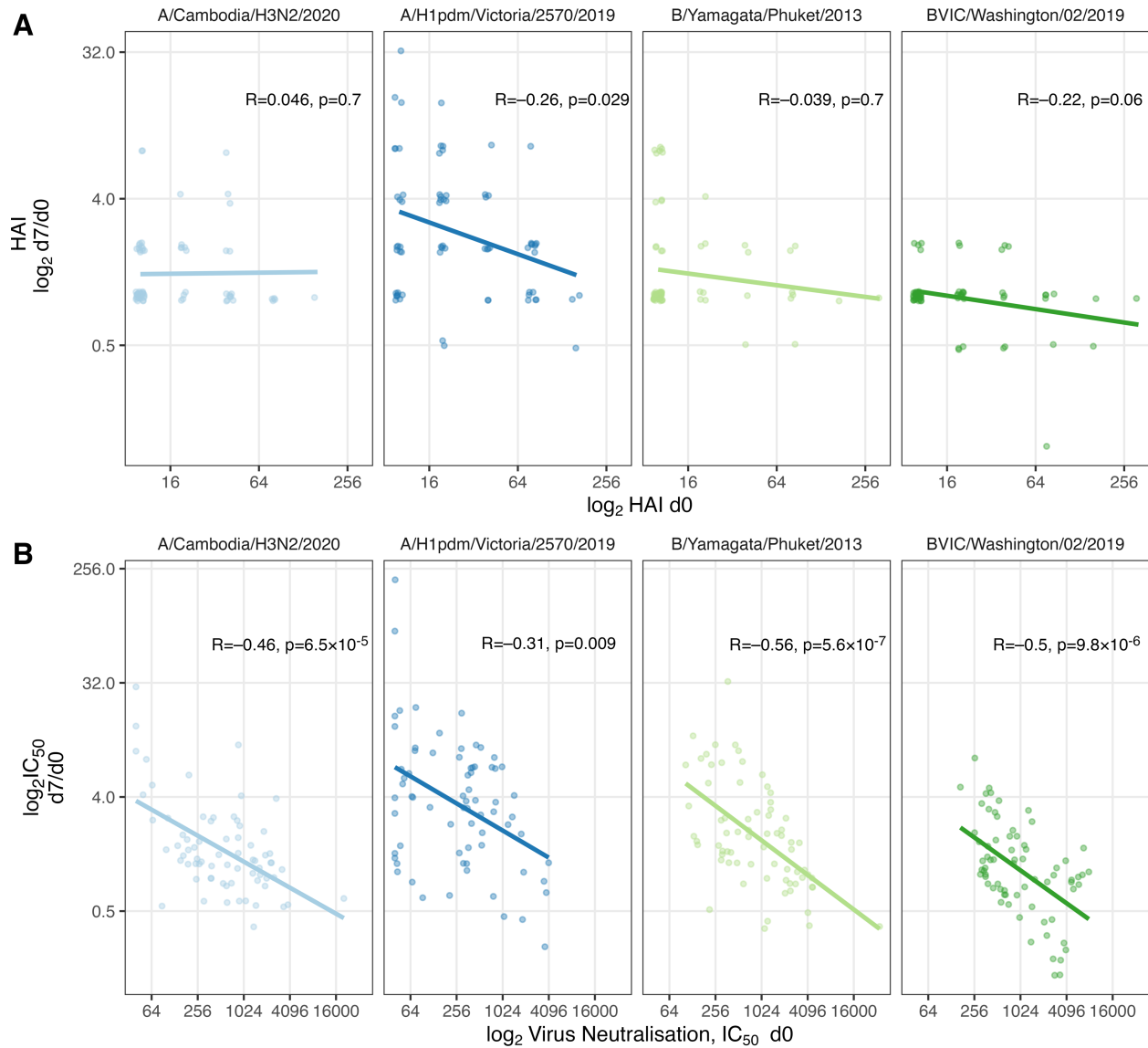
Fig 3. Pre-existing antibody inhibits subsequent vaccine responses (A & B) Log 2 fold changes of peak titres (d7/d0) plotted against d0 titres for HAI (A) or LV-N (B). In (A & B), Spearman correlation coefficients and P values are shown, and a fit line from linear regression plotted.
