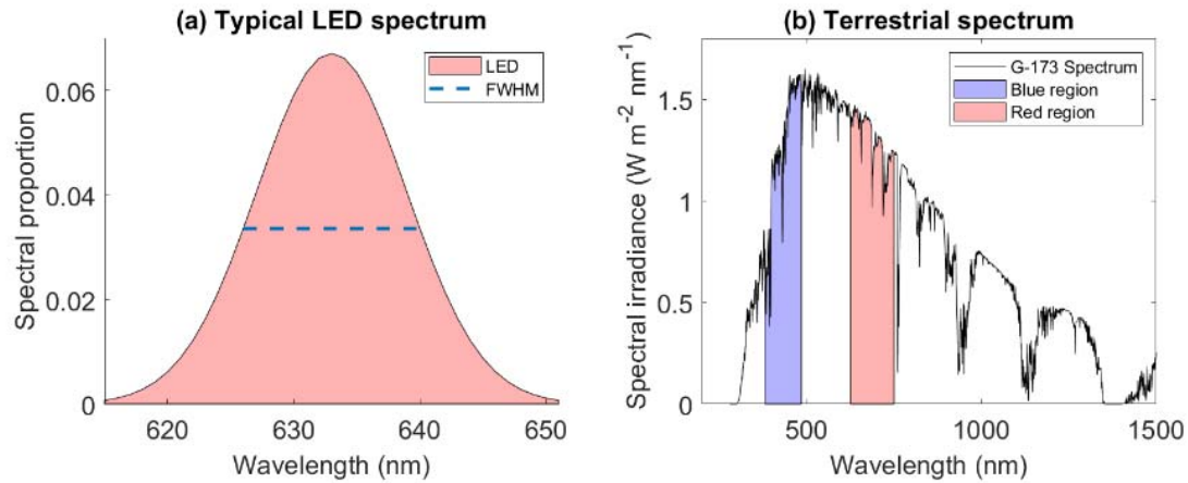
Figure 1 - (a) Spectrum for a red LED with \lambda_c = 633 nm and FWHM = 14 nm, (b) Terrestrial solar spectrum with violet / blue band (380 - 485 nm) and red band (625 - 750 nm) highlighted
