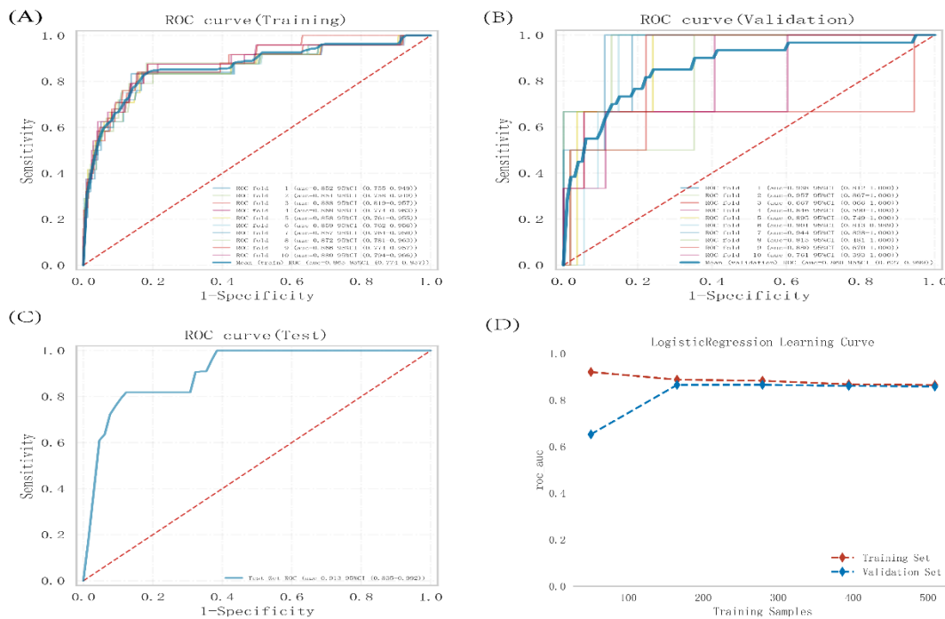
Fig 3. Logistic regression model training, validation, and testing. (A) Training sets ROC and AUC and (B) validation sets ROC and AUC. Training and cross-validation of 10% of COPD patients. Solid lines of different colors represent 10 different results. (C) Test set ROC and AUC. Test results for 30% of COPD patients. (D) Learning curve. The red dashed line represents the training set and the blue dashed line represents the validation set. The values are expressed in terms of average and 95% CI.
