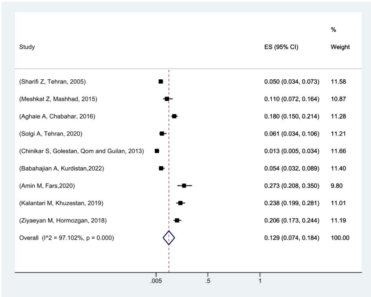
468 Figure 2. Pooled prevalence of positive ELISA test for West Nile virus in Iran based on the random 469 effects model. The midpoint of each line segment shows the prevalence estimate, the length of the line 470 segment indicates the 95% confidence interval in each study, and the diamond mark illustrates the pooled 471 prevalence.
