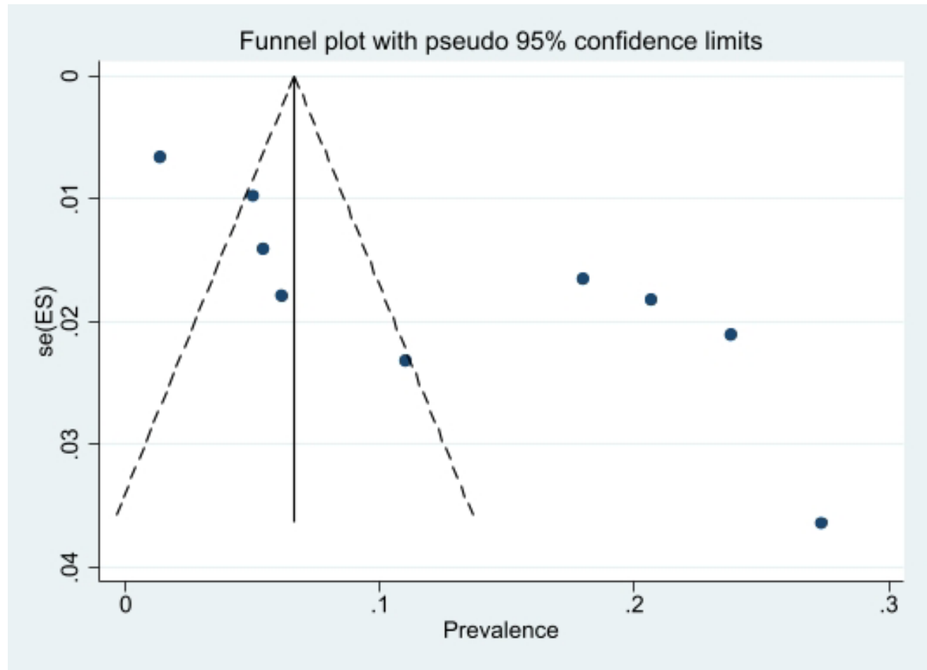
Figure 4. Funnel plot of the prevalence positive ELISA test in the selected studies.
