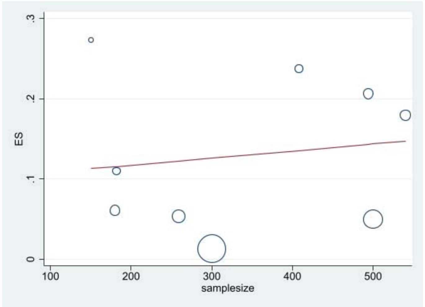
Figure 5. Meta-regression plot of prevalence of West Nile virus and sample size of study.
