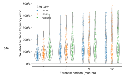
Figure 5—figure supplement 3. Distribution of total absolute clade frequency errors summed across clades per future timepoint for simulated A/H3N2-like populations.
