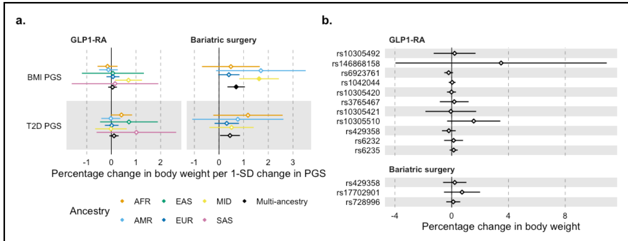
Figure 2 | Effect of 15 genetic exposures on body weight changes associated with GLP1-RA treatment and bariatric surgery.
