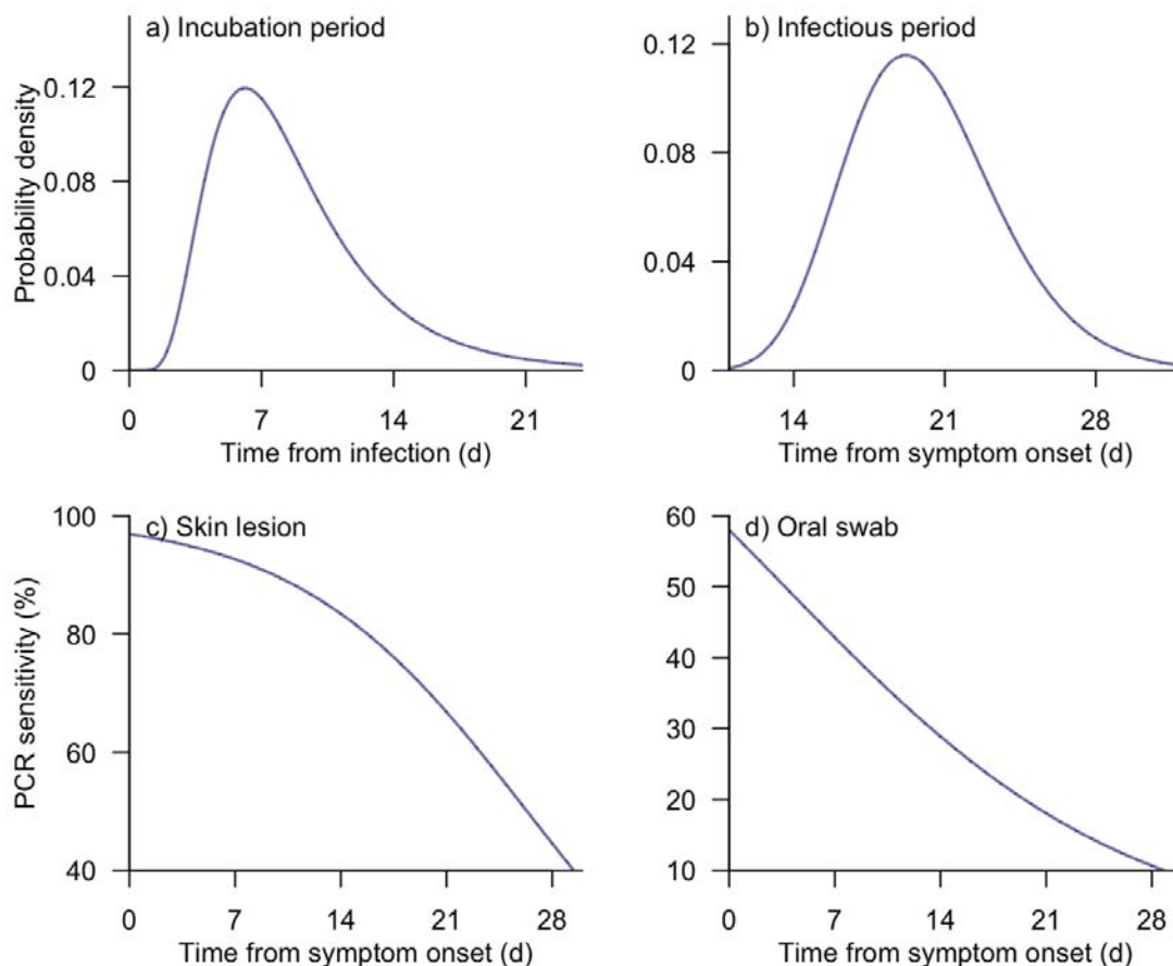
Figure 1. Distribution of the parameters for the model of disease progression. Probability density for incubation period (a) and time from symptom onset to loss of infectiousness (b) 1 . Sensitivity of PCR test using samples of skin lesions (c) and oropharyngeal samples (d) over time 14 . Note that the time points with relatively low probability density (a-b) or sensitivity (c-d) may not be fully displayed.
