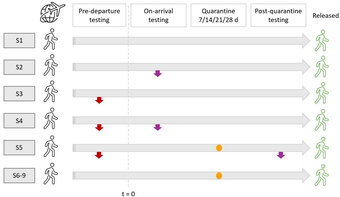
Figure 2. Descriptions of Strategies 1–9 and outcomes. Red arrows in Strategy 3–5 represent infected individuals detected by pre-departure PCR tests and thereby not permitted entry. Purple arrows in Strategy 2, 4, and 5 represent infected individuals detected by PCR tests or those who lost infectiousness while awaiting testing results. These individuals would not be able to infect others upon release into the community. Orange dots in Strategy 5–9 denote undiagnosed infections who lost infectiousness during quarantine. Strategies 6–9 are presented together in the last row as they differ only in quarantine duration. The time scale ( ) is the time from departure for all the travellers.
