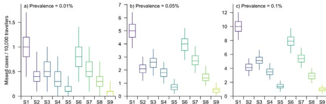
Figure 4. Number of missed cases per 10,000 travellers. Summary statistics include medians, interquartile ranges (IQRs), and 95% confidence intervals (CIs) for Strategy 1–9 when the disease prevalence was 0.01% (a), 0.05% (b), or 0.1% (c) in the country of origin.
