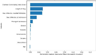
Feature Importances with Permutation
