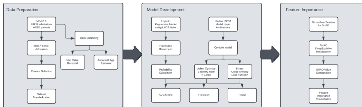
Figure 1 Flow Chart of Data Preparation, Model Development and Feature Importance Analysis
