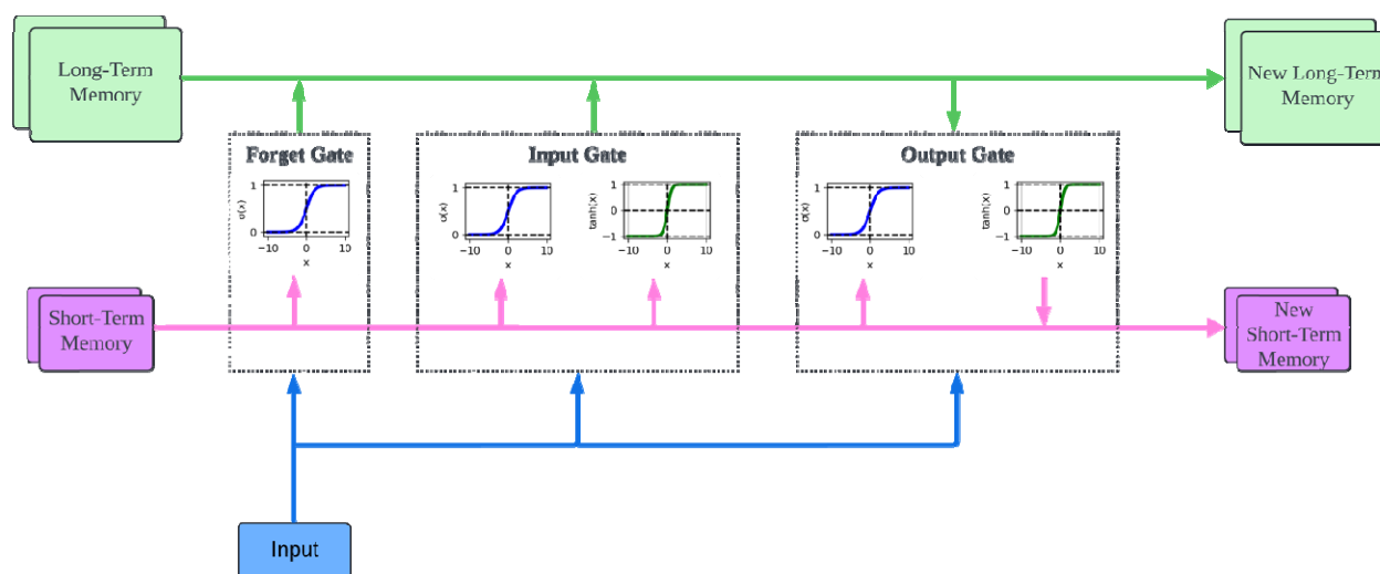
Figure 2 Long Short-Term Memory Neural Networks
