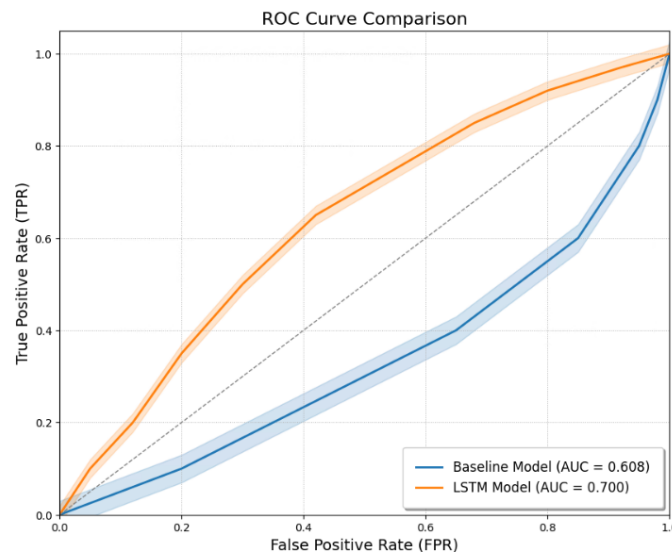
Figure 4 AUC Comparison of Logistic Regression and LSTM
