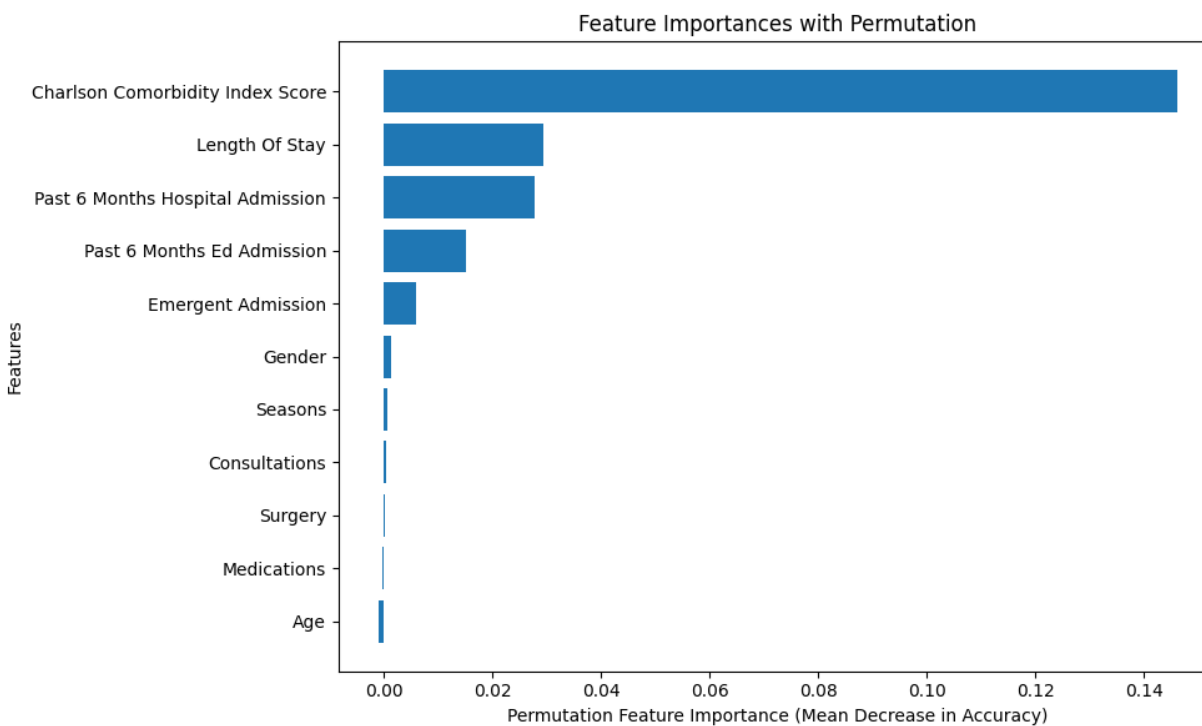
Figure 5 Permutation Analysis
