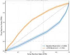
ROC Curve Comparison
