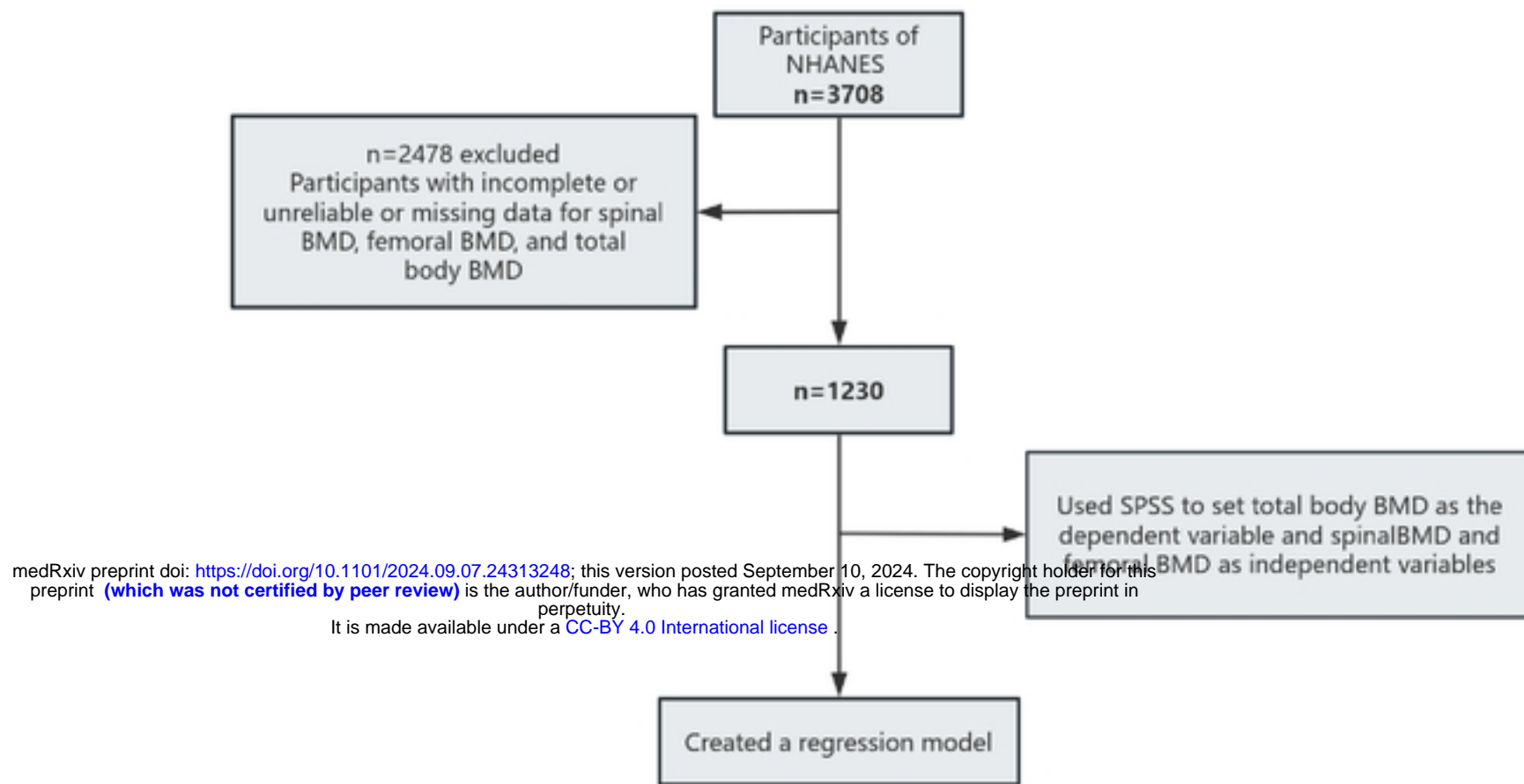
Figure 2 Flowchart for creating the linear regression model
