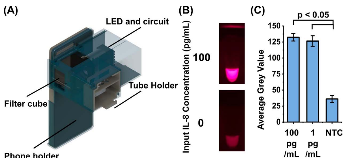
Figure 4. Smartphone-based detection device. (A) The device was 3D printed to enclose the optical module (red light-emitting diode (LED) and circuit, and filter cubes) and enable the mounting of the smartphone and the sample tubes. (B) With the red LED as the excitation resource and the excitation filter to illuminate the reaction tubes, two representative tube images were taken using the smartphone with emission filter, shown with 100 pg/mL and 0 pg/mL IL-8 concentration. (C) The smartphone detection showed distinguishable signal from 100 pg/mL and 1 pg/mL IL-8 target to NTC ( n = 3 , p < 0.05 ). Data represented in (C) as mean \pm SD.
