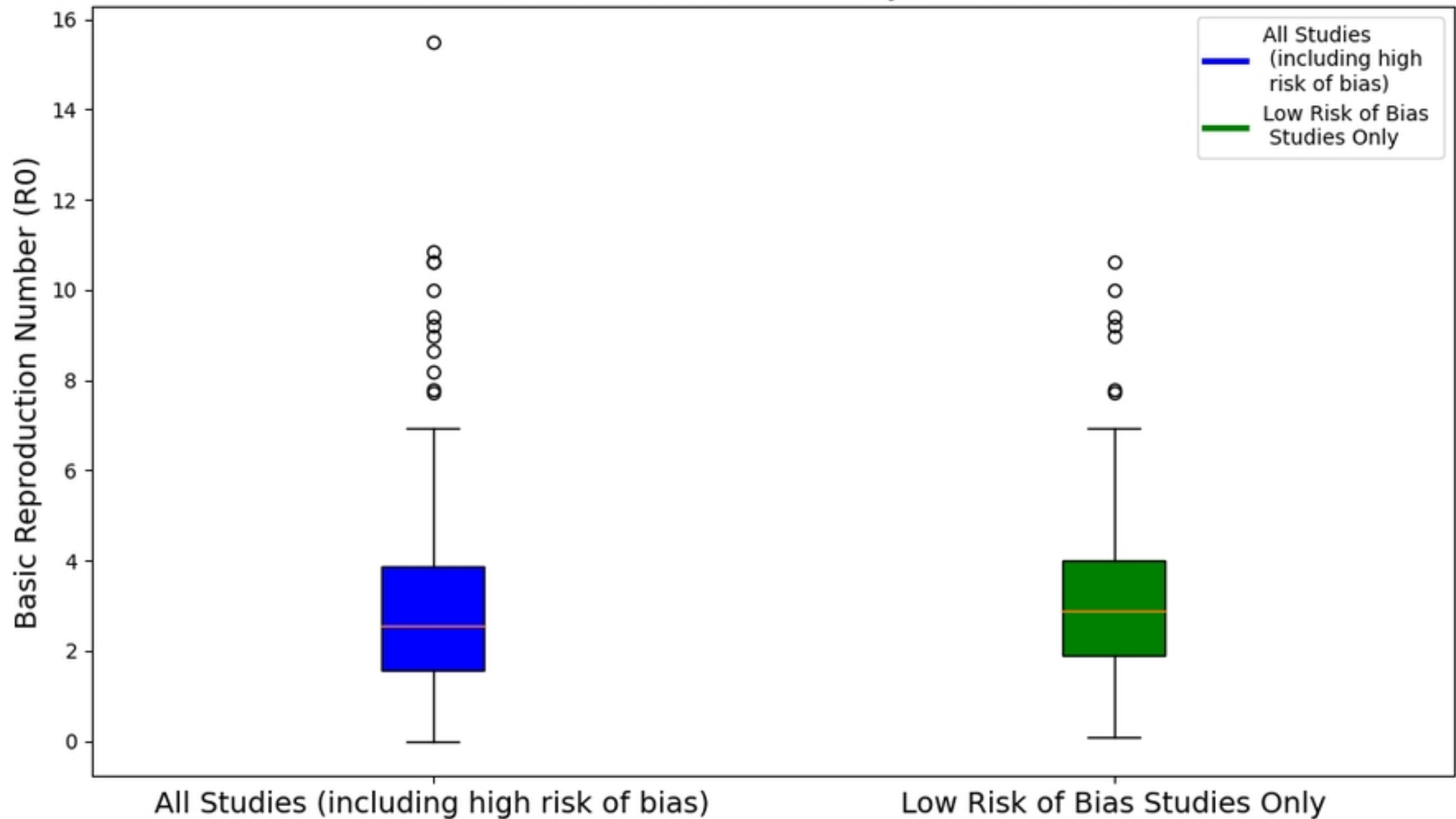
R0 of all 270 studies Vs R0 of only low risk studies
