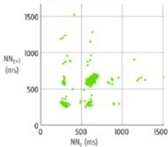
POINCARÉ PLOT
