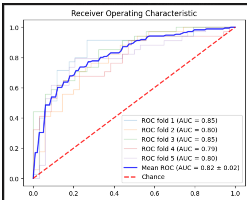
Figure 3 - Area under the curve for the FC model with balanced classes
