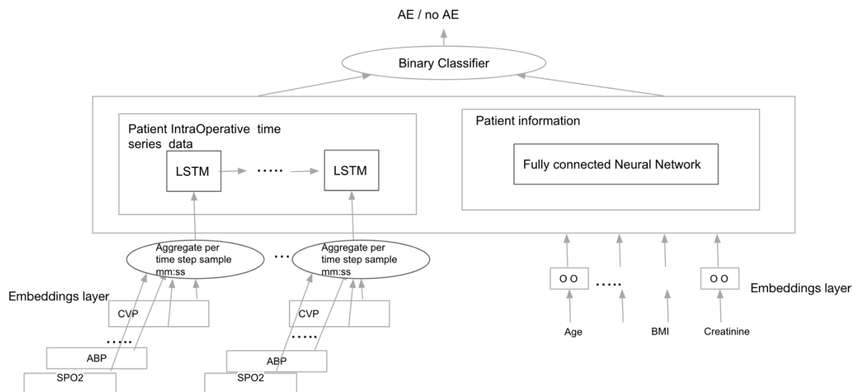
Figure 1 - Architecture of Fully Connected and LSTM Networks
