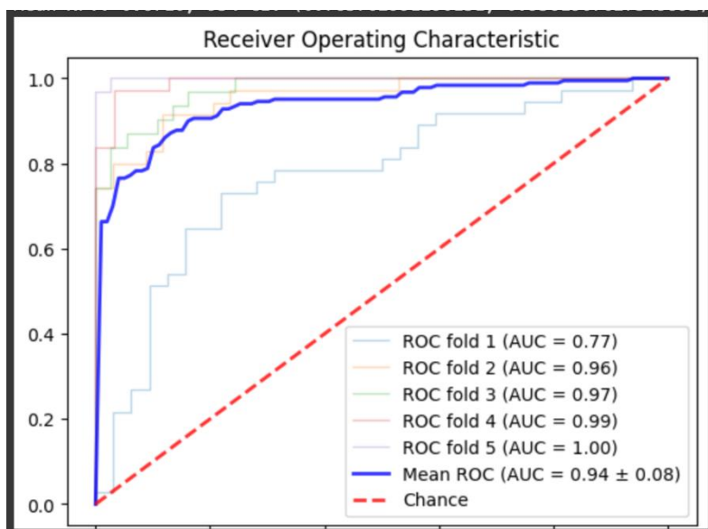
Figure 5 - Area under the curve for the FC + LSTM model with only impactful time series features
