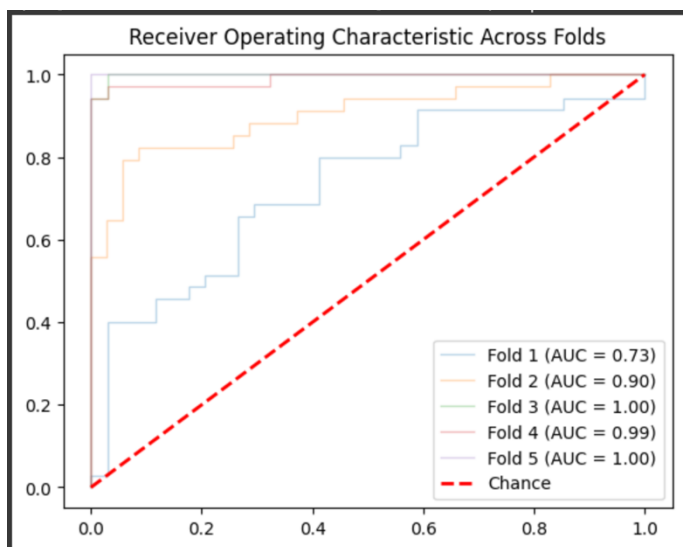
Figure 2 - Area under the curve for the FC + LSTM model with balanced classes
