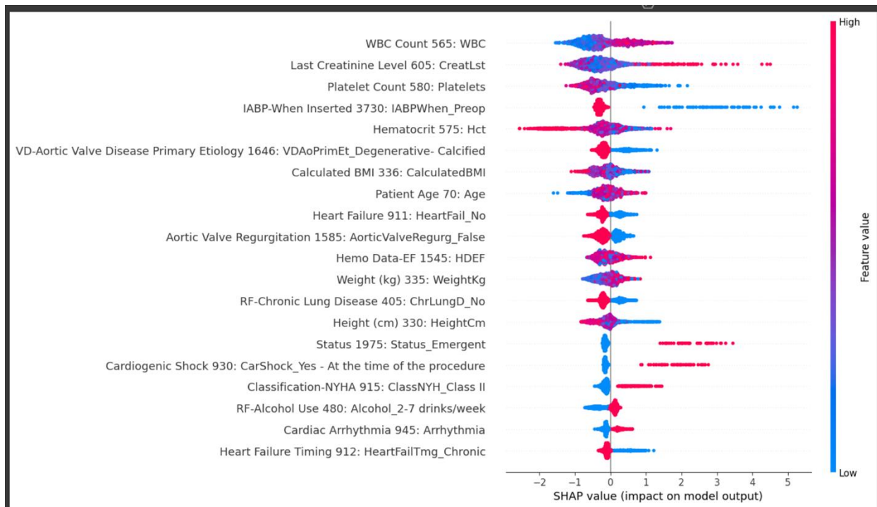
Figure 7 - Absolute SHAP Values for Top 20 Predictive Features in the XGBoost Model
