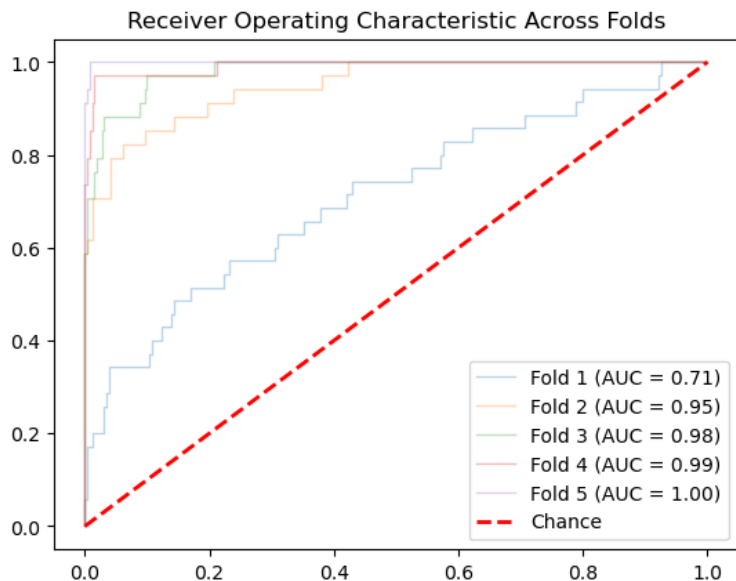
Figure 3 - Area under the curve for the FC + LSTM model with unbalanced classes
