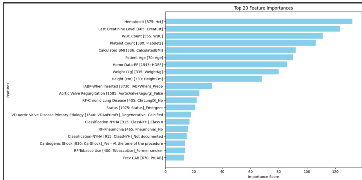
Figure 6 - Top 20 most predictive features in static variables according to XGBoost
