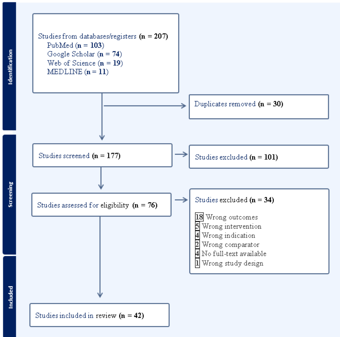
Fig 1. PRISMA Diagram
