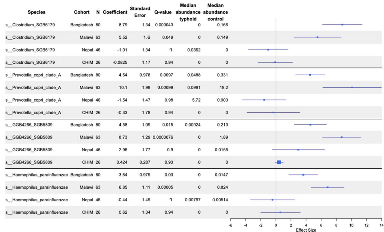
Figure 2: Forest plot of species that significantly differed between household contacts and typhoid fever participants in at least two endemic countries. Results from all three endemic countries and the CHIM cohort are shown for context. CHIM maaslin2 analysis only included species that were significantly associated in at least two of the endemic country sites. Species are labelled with their GTDB identifier, note that 's__ GGB4266_SGB5809' refers to a proposed novel genus/species of Veillonellaceae.
