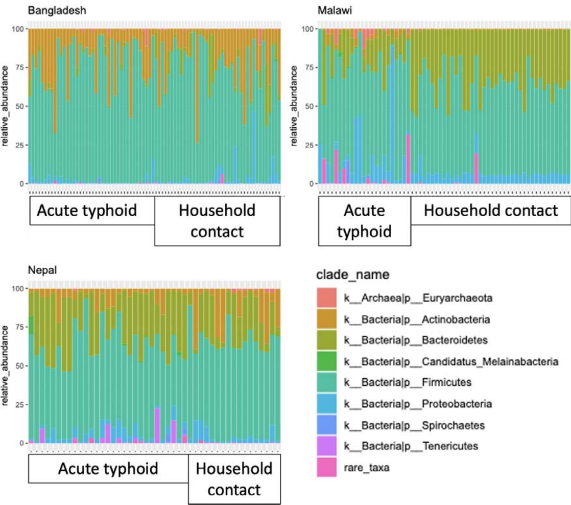
Supplementary Figure 4: Bar chart showing the prevalence of eight common phyla in acute typhoid patients and healthy household contacts, for each study site.
