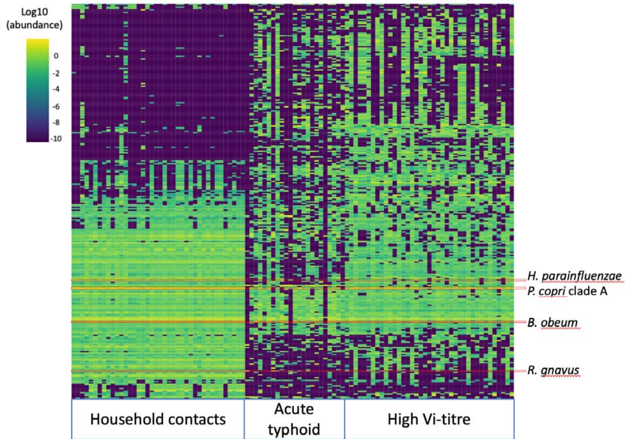
Figure 4: Heatmap of the abundance of the 400 most abundant species in household contacts, acute typhoid fever cases and high Vi-titre participants from Malawi. The columns are sorted by participant group, rows are sorted by hierarchical clustering across all samples.
