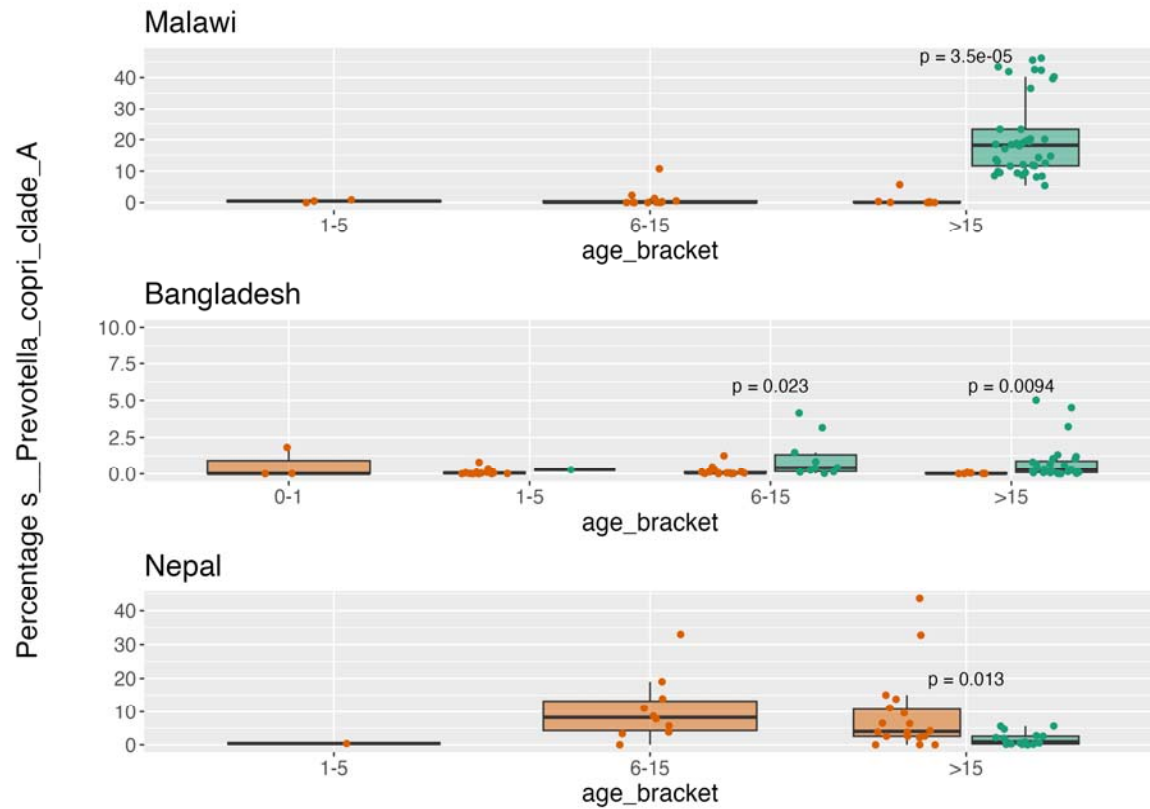
Supplementary Figure 5: Prevalence of Prevotella copri clade A across age brackets in Malawi, Bangladesh, and Nepal.
