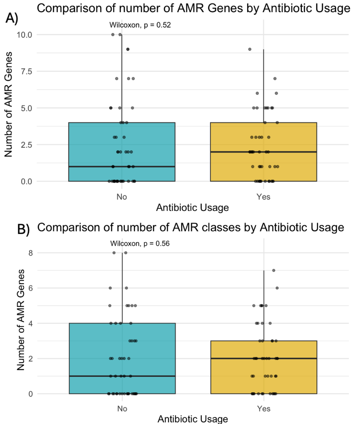
Supplementary Figure 14: Comparison of A) the number of AMR gene and B) the number of AMR gene classes identified in participants from all three sites who did and did not report antibiotic usage prior to sampling
