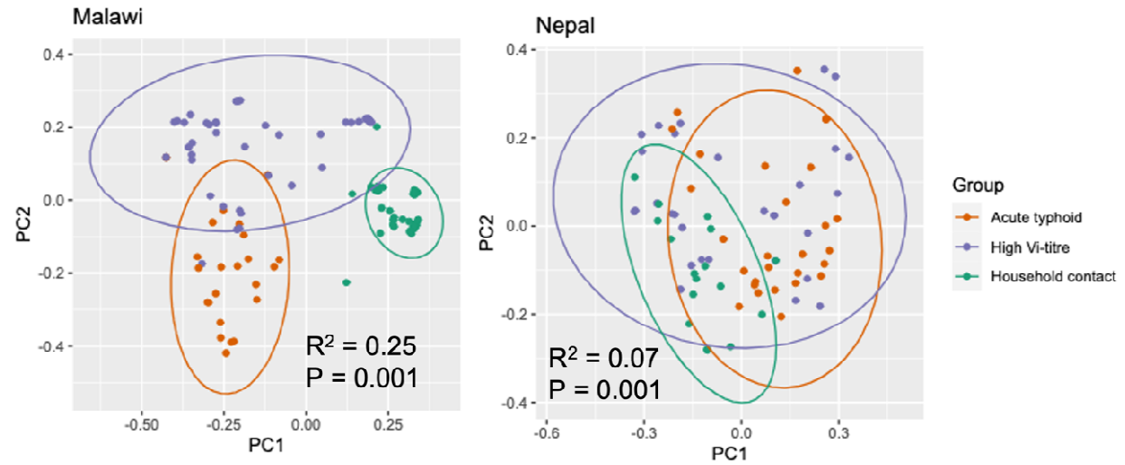
Supplementary Figure 10: Beta diversity of acute typhoid fever, high Vi-titre participants, and household contacts from Malawi and Nepal
