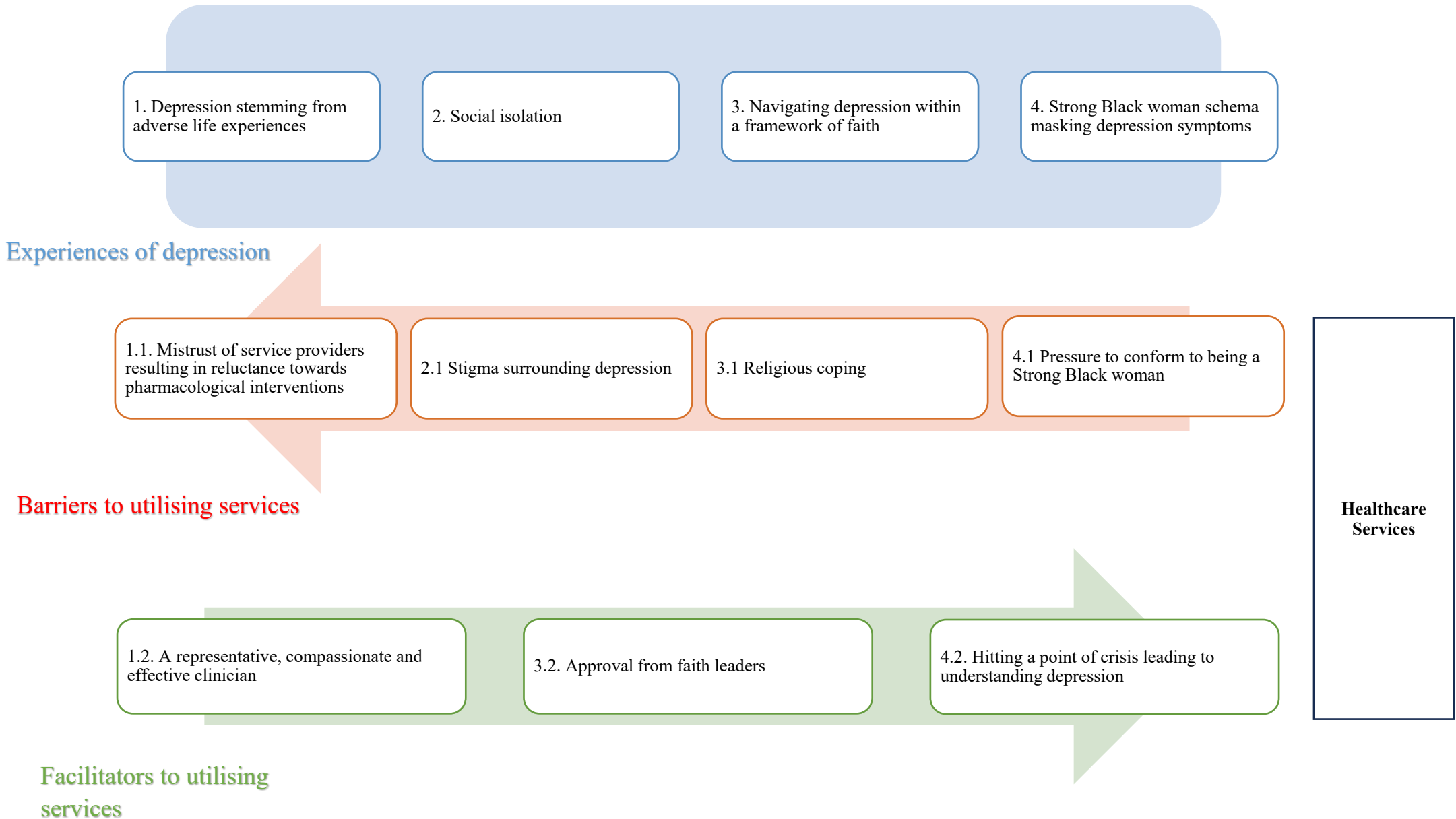
Figure 3: Logic model
