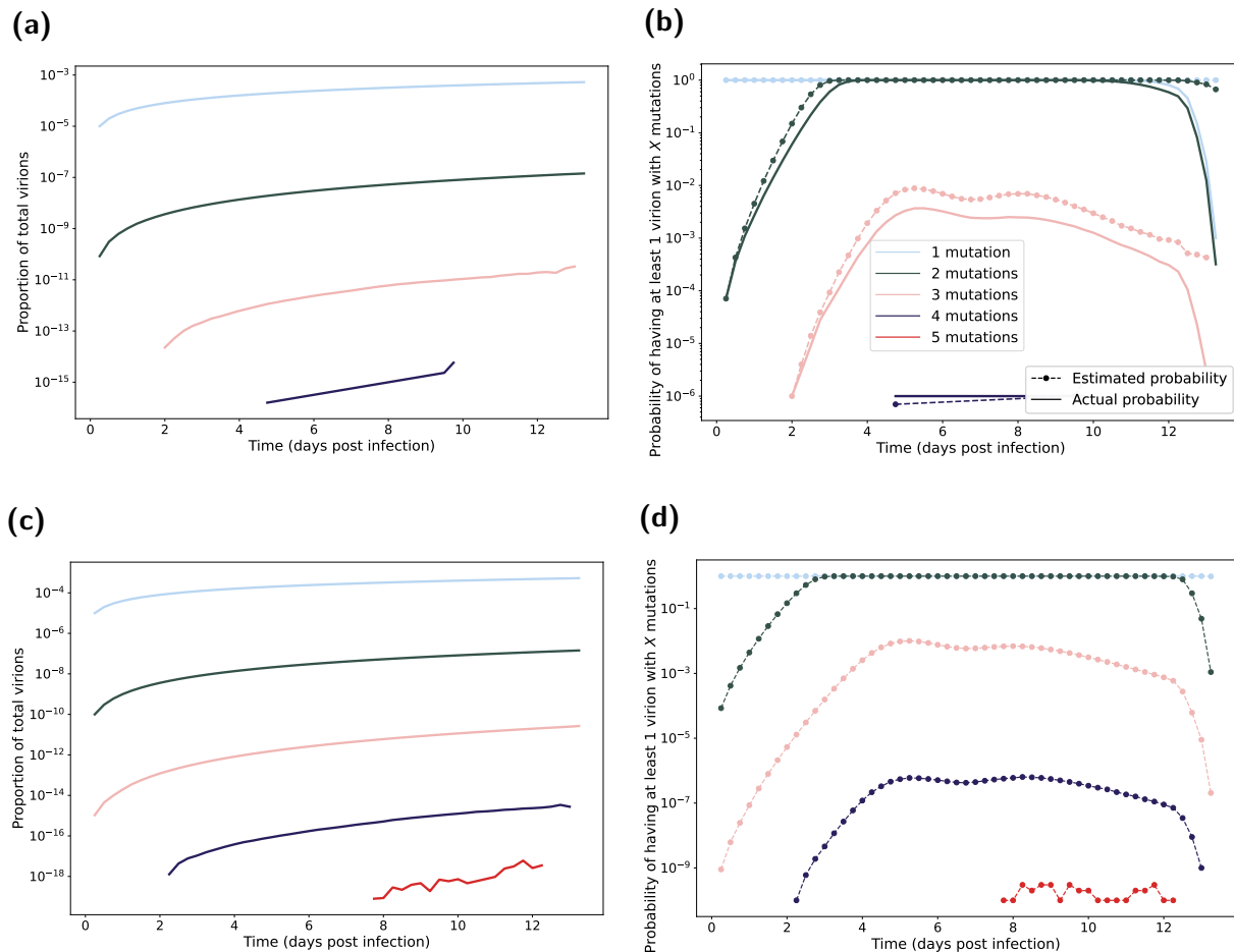
Fig. 7. Mutated virion statistics with respect to time elapsed post infection, computed from BPM realisations. Line shading corresponds to the number of mutations (one mutation the lightest shading through to five mutations being the darkest shading). In all BPM simulations we fixed the probability of mutation at 10^{-5} per replication. In panels (a&b), each realisation had an initial viral load of 10^6 . We ran 1000 realisations of each of the 1000 posterior parameter sets (Fig. 4). In panels (c&d), each realisation had an initial viral load of 10^6 \times 10^6 . We ran one realisation of each of the 1000 posterior parameter sets (Fig. 4). (a,c) Proportion of total virions with the specified amount of mutations. There were a very small proportion of virions that have the required number of mutations to achieve droplet transmission (three or more mutations). (b,d) Probability of having a mutation strain. We present the estimated probabilities as the dashed lines with circle markers. We present the actual probabilities as solid lines. Probability estimate derivation follows that given in Section 2.2. The estimated probabilities are a clear upper bound on the true probabilities. Depending on the number of mutations in the initial infecting virions, there was a low probability of achieving the required number of mutations near the beginning on the infection lifespan (which would allow more replication of the mutant strains).
