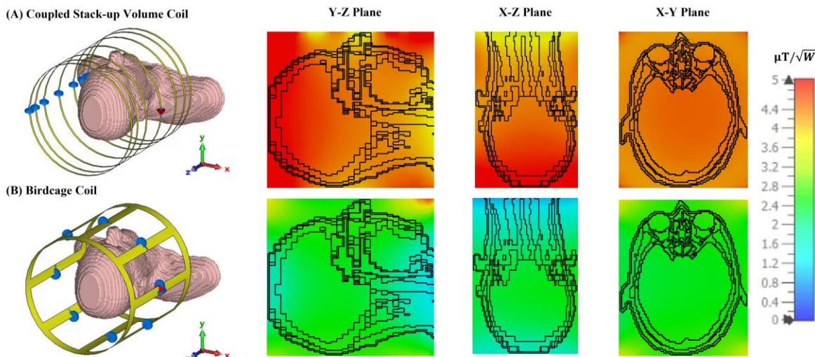
488 489 Figure 10. Simulated B1 efficiency and field distribution in three orthogonal planes: Comparison 490 between the (A) proposed coupled stack-up volume coil and the (B) birdcage coil loaded with a 491 human head phantom.
