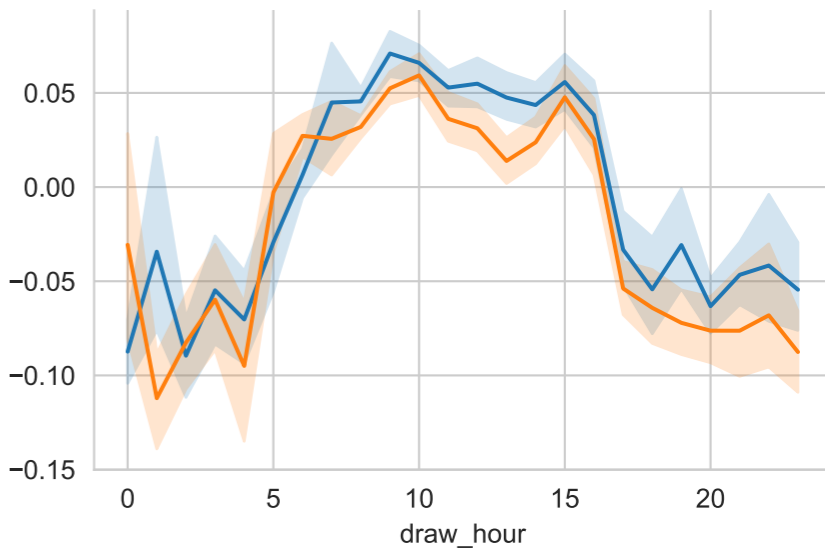
component = UMAP_5
