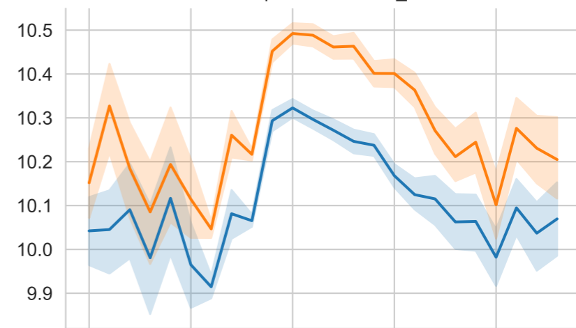
component = UMAP_5
