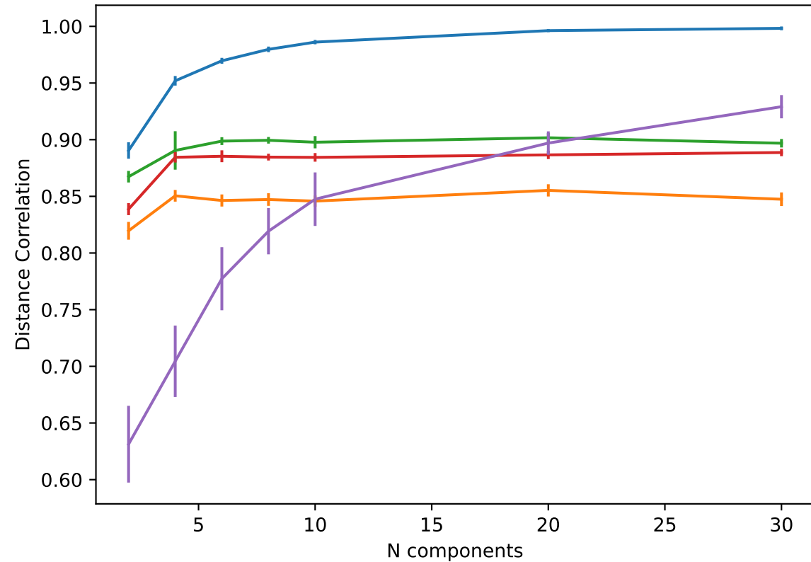
Distance Correlation
