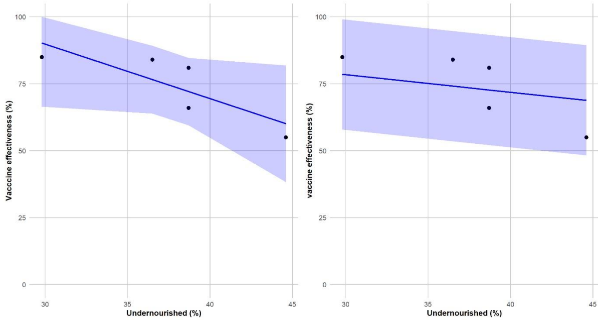
Figure 2. Model fit and 95% confidence intervals Model-1 standard linear model (left), Model-2 constrained linear model (right)
