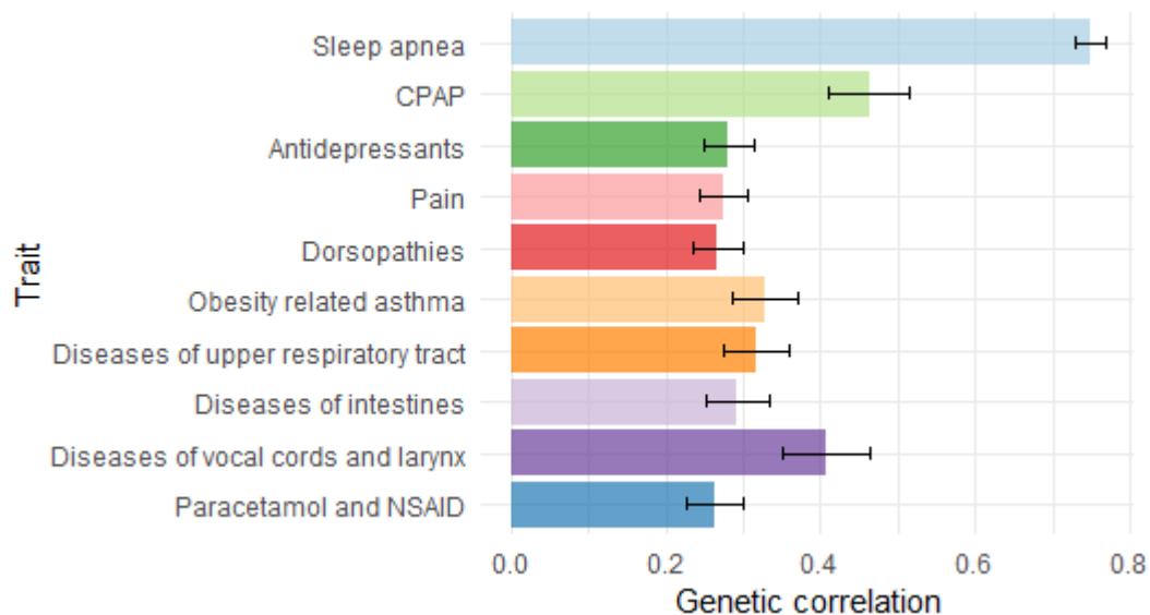
Figure 4. Genetic correlation with clinical electronic health record phenotypes. Genetic correlations between obstructive sleep apnea (OSA diagnosis + body mass index under 30 kg/m 2 ) and its most significant correlates calculated using LDSC regression utilizing data from FinnGen.
