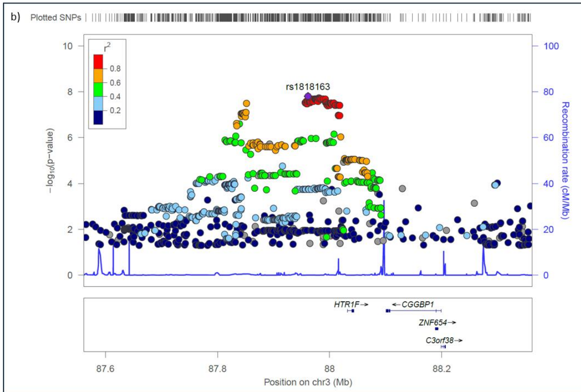
Figure 1. a) A Manhattan plot depicting results from a genome-wide association study (GWAS) investigating genetic variants associated with obstructive sleep apnea in individuals whose body mass index is under 30 (20,413 cases and 443,463 controls). The notable peak coincides with the genomic location of the HTR1F gene. b) Regional association of HTR1F shows association signal intronic at the HTR1F locus.
