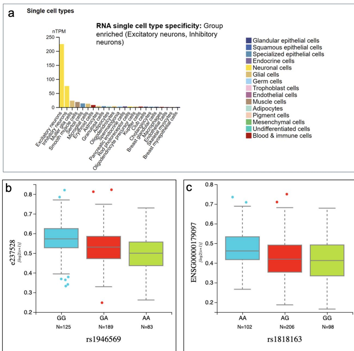
Figure 2. HTR1F expression profile. HTR1F displayed higher expression levels in specific neuronal cell types compared to others, suggesting potential roles in the excitatory or inhibitory functions of neurons. b) eQTL lead variant on exon HTR1F exon expression ( r^2 = 0.8 with rs1818163) and c) eQTL of rs1818163 on HTR1F gene expression.
