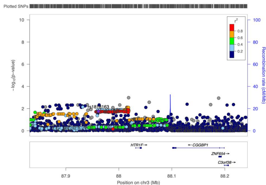
Supplementary Figure 2. Regional association plot of HTR1F region in Estonian Biobank BMI < 30.
