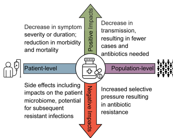
Figure 1: Schematic of individual and population-level harms and benefits of antibiotic use. The horizontal axis describes the individual (patient-level) and population-level impacts and the vertical axis describes the benefits (positive impacts) and harms (negative impacts) of antibiotic usage.
