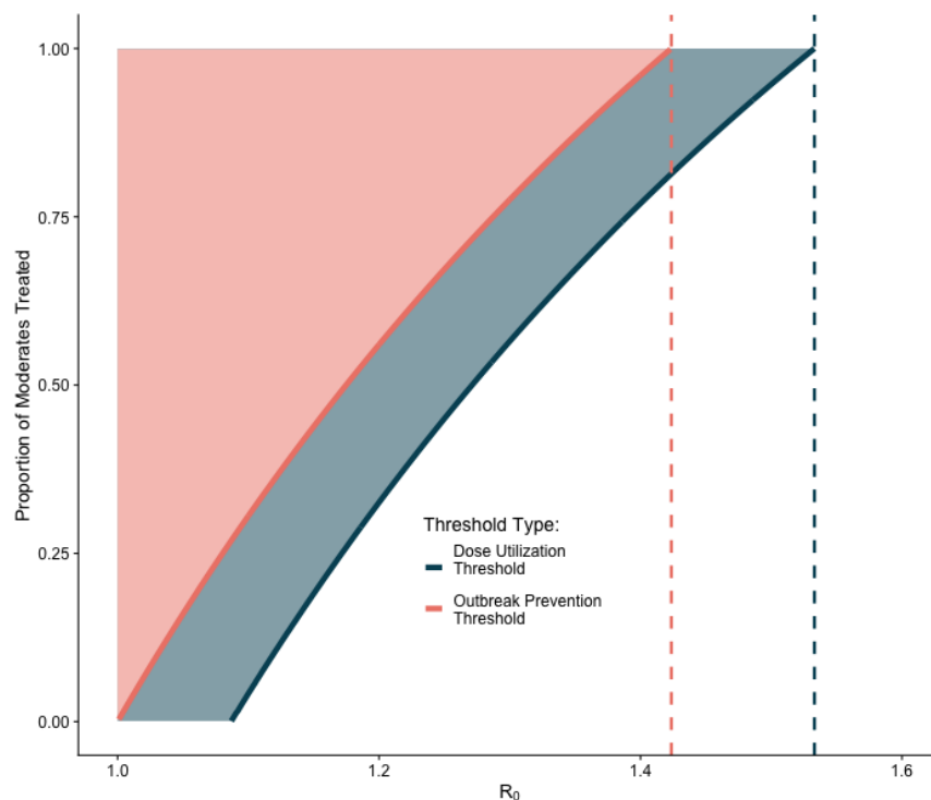
Figure 4: Plot of the threshold values for dose reduction (DUT) and outbreak prevention (OPT), by \mathcal{R}(q=0) , for each proportion of moderates treated ( M_{abx} ). For a each value of \mathcal{R}(q=0) , the pink curve shows the OPT of \mathcal{R}(q=0) and M_{abx} , the shaded region above the curve shows all combinations of \mathcal{R}(q=0) and M_{abx} in which treating moderate infections reduces the effective reproductive number, \mathcal{R}(q) , below 1. The dotted red line indicates \mathcal{R}_{opt} for cholera. The blue curve shows the DUT of \mathcal{R}(q=0) and M_{abx} , the shaded region above the curve shows all combinations of \mathcal{R}(q=0) and M_{abx} in which fewer doses are given overall with expanded treatment. The dotted blue line indicates \mathcal{R}_{dut} for cholera. Outside of these regions, in the white space, there is no outcome improvement.
