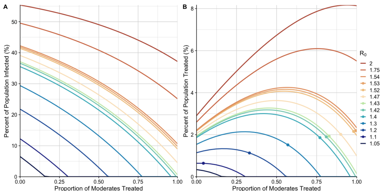
Figure 3: The final size (A) and proportion of total population treated (B) plotted against M_{abx} in a cholera outbreak for different values of \mathcal{R}(q = 0) . Each curve corresponds to a different value of \mathcal{R}(q = 0) , representing different outbreak scenarios of varying severity and transmissibility. (A) the percent of the population infected, regardless of severity of infection or treatment status, over an outbreak ( r_\infty ). (B) the percent of the population that receive antibiotics, including moderate and severe infections, over the course of an outbreak ( r_{abx\infty} ). Dots indicate the proportion of moderates that need to be treated to cross the Dose Utilization Threshold (DUT), for each value of \mathcal{R}(q = 0) . Lines without points indicate that \mathcal{R}(q = 0) > \mathcal{R}_{dut} .
