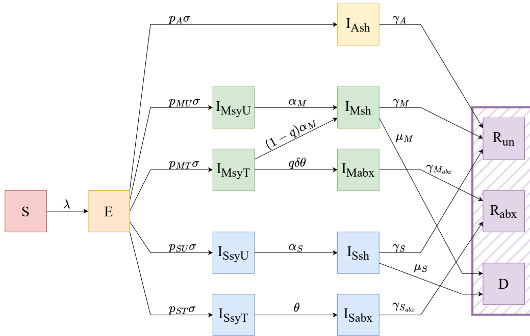
Figure 2: Compartmental model of cholera transmission dynamics. Each compartment represents a different epidemiological class. All individuals begin in the susceptible class ( S ), and become exposed ( E ) at rate \lambda . From E , individuals become infectious ( I ) and, based on their symptoms, follow one of five different paths (Supplement 4 further describes rates p_{A\sigma} , p_{MU\sigma} , p_{MT\sigma} , p_{SU\sigma} , p_{ST\sigma} ). Post-infection, individuals are removed in one of three ways (purple hatching: R_{un} , R_{abx} , D ). Breaking down the transition from exposure to infectiousness, exposed individuals become asymptotically infected ( I_{Ash} ) at rate p_{A\sigma} , are never eligible for treatment, and recover at rate \gamma_A to the recovered, untreated compartment ( R_{un} ). Exposed individuals become infected with moderate symptoms ( I_{MsyT} or I_{MsyU} ) at rate p_{MT\sigma} or p_{MU\sigma} depending on whether or not they seek treatment. Moderately infected individuals who do not seek treatment ( I_{MsyU} ) recover from symptoms at rate \alpha_M and continue to shed ( I_{Msh} ) until they fully recover at rate \gamma_M to the recovered, untreated compartment ( R_{un} ), or they die at rate \mu_M , moving to the dead compartment ( D ). Moderately infected individuals who seek treatment ( I_{MsyT} ) may or may not receive treatment based on the model scenario. Treatment seeking patients with moderate infections receive treatment and recover from symptoms at rate q\delta\theta or do not receive treatment and recover from symptoms at rate (1-q)\alpha_M . Moderate infections who receive treatment continue to shed ( I_{Mabx} ) for a shorter duration than those not receiving treatment, and fully recover at rate \gamma_{Mabx} to the recovered, treated compartment ( R_{abx} ). Treatment seeking patients with moderate infections who do not receive treatment recover from symptoms and continue to shed ( I_{Msh} ) until they fully recover at rate \gamma_M to the recovered, untreated compartment ( R_{un} ), or they die at rate \mu_M , moving to the dead compartment ( D ). Exposed individuals become severely infected ( I_{SsyU} or I_{SsyT} ) at rate p_{SU\sigma} or p_{ST\sigma} depending on whether or not they seek treatment. Severely infected individuals who do not seek treatment ( I_{SsyU} ) recover from symptoms at rate \alpha_S and continue to shed ( I_{Ssh} ) until they fully recover at rate \gamma_S to the recovered, untreated compartment ( R_{un} ), or they die at rate \mu_S , moving to the dead compartment ( D ). All individuals with severe infections who seek treatment ( I_{SsyT} ) receive treatment with antibiotics at rate \theta . Those with severe infections who receive treatment continue to shed ( I_{Sabx} ); however, they remain hospitalized until symptoms resolve and therefore do not contribute to transmission. They then fully recover at rate \gamma_{Sabx} to the recovered, treated compartment ( R_{abx} ). Full model equations can be found in Supplement 4.
