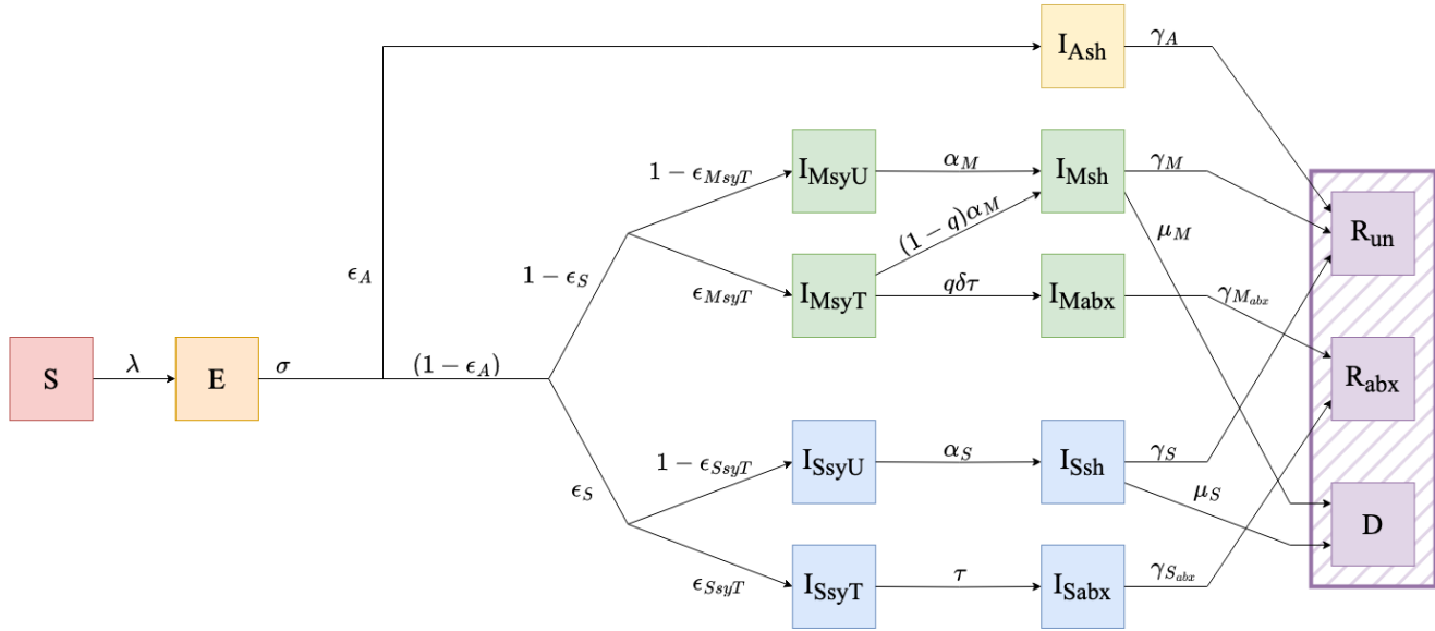
Figure S1: Model diagram with detailed parameterization of pathways between exposure and infection.
