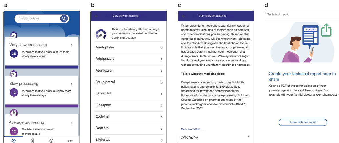
Figure 5: Overview of the 'Gen en Geneesmiddel' app (translated from Dutch). a) Main menu, where five categories can be selected: 'poor', 'intermediate', 'normal' and 'ultrarapid' metabolism and 'other processes'. b) A personalized list of medication in the 'poor metabolism' category. c) Explanation of the predicted metabolism of brexpiprazole. d) The pharmacogenetic profile can be saved or shared from the app.
