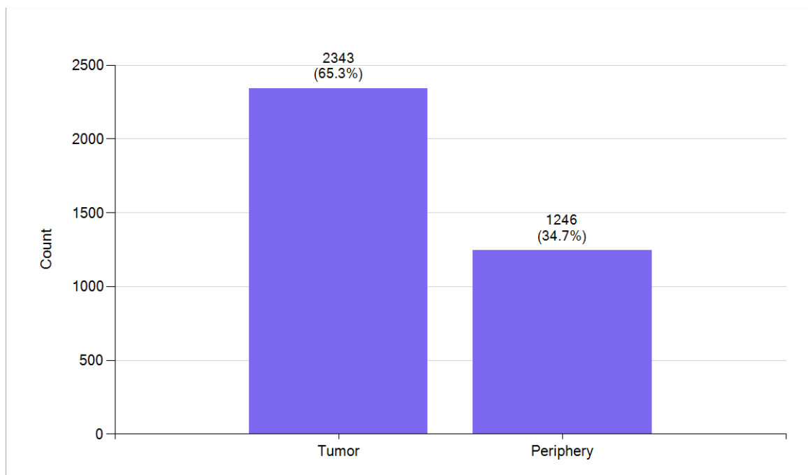
Figure 1: GSE84465 contains 2343 GBM tumor single cells and 1246 periphery single cells.
