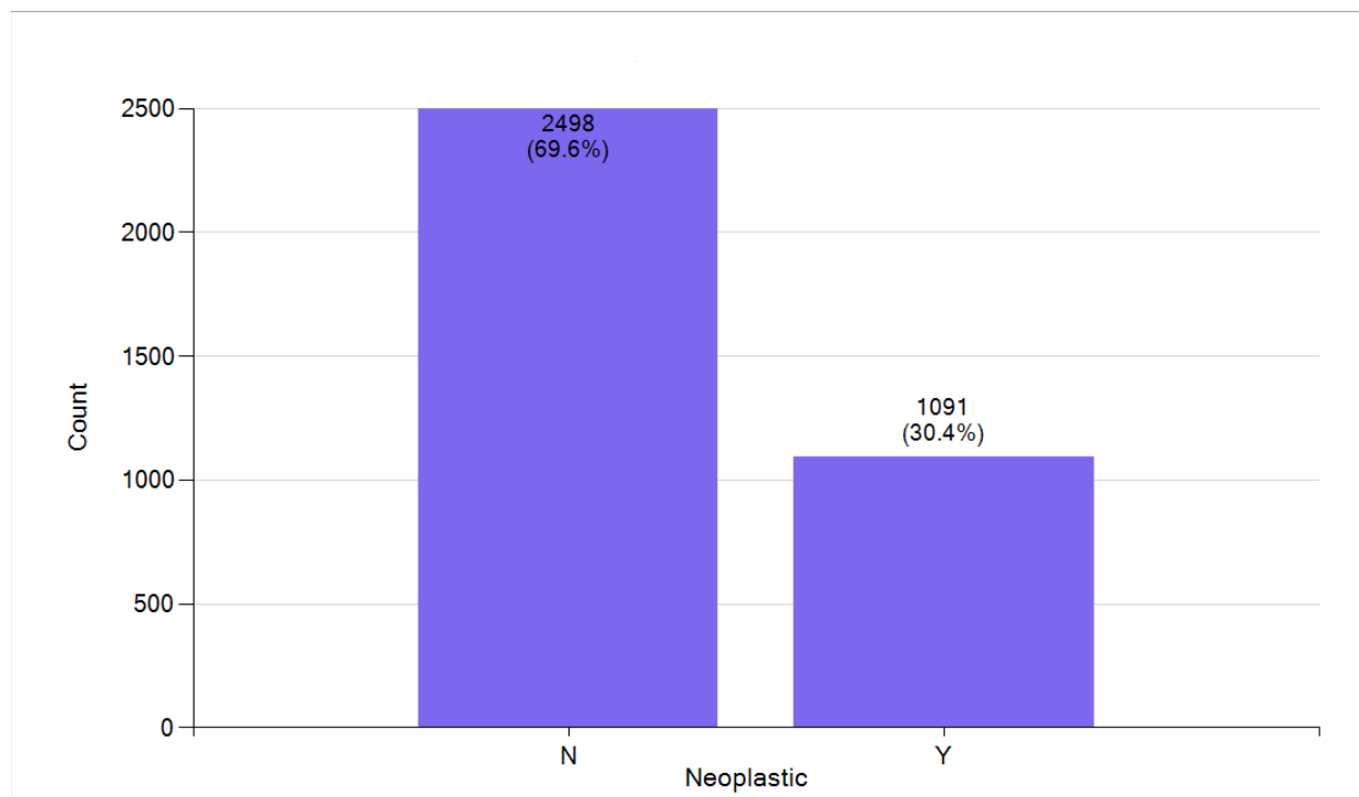
Figure 3: GBM non-neoplastic and neoplastic single cells.
