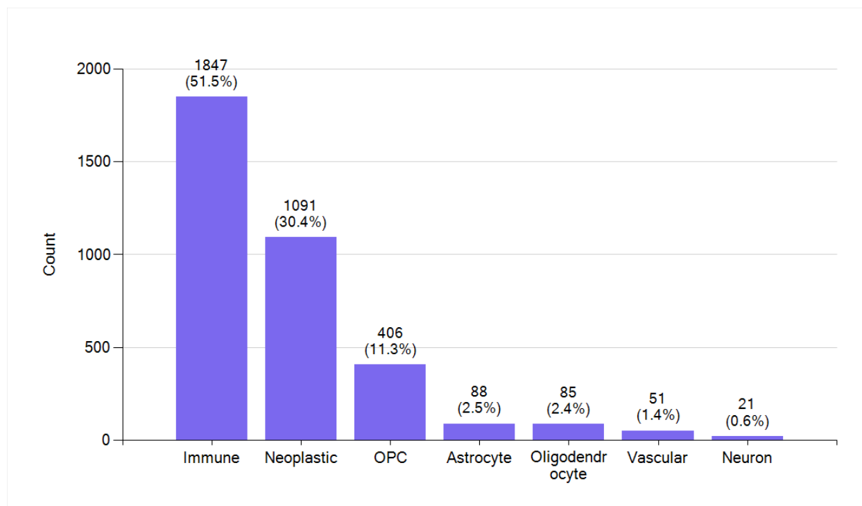
Figure 2: GSE84465 includes seven different cell types. Oligodendrocyte progenitor cells (OPC) are a subtype of glia in the central nervous system named for their essential role as precursors to oligodendrocytes and myelin.
