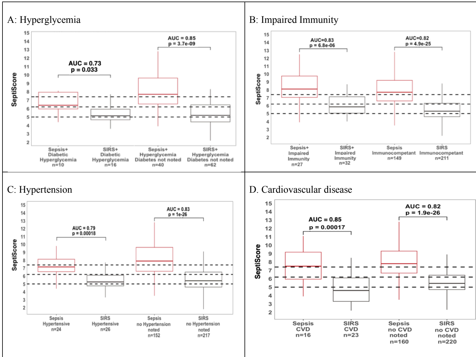
Figure 1: Box and whisker plots of SeptiCyte RAPID performance in patients with (A) hyperglycemia, (B) impaired immunity, (C) hypertension, (D) cardiovascular disease, (E) kidney disease, (F) obesity.
