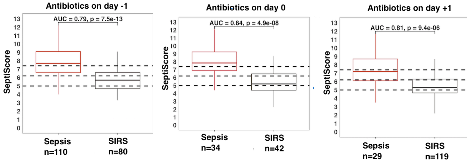
Figure 4: Box and whisker plots of the influence of antibiotic treatment (Abx) initiation time on SeptiCyte RAPID performance. The day of blood draw is defined as day 0. (A) treatment initiated -1 days to 0 days relative to blood draw; (B) antibiotic treatment initiated on the same day as blood draw. (C) antibiotic treatment initiated +1 day after blood draw.
