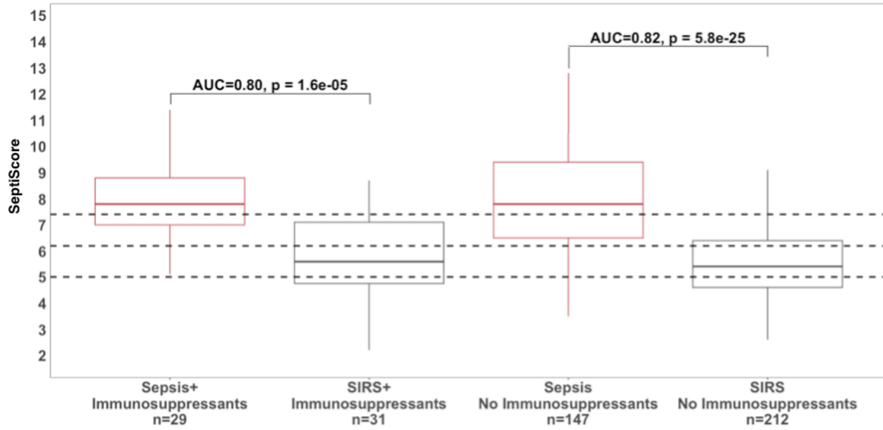
Figure 3: Box and whisker plot of SeptiCyte RAPID performance for patients treated vs. not treated with immunosuppressants.
